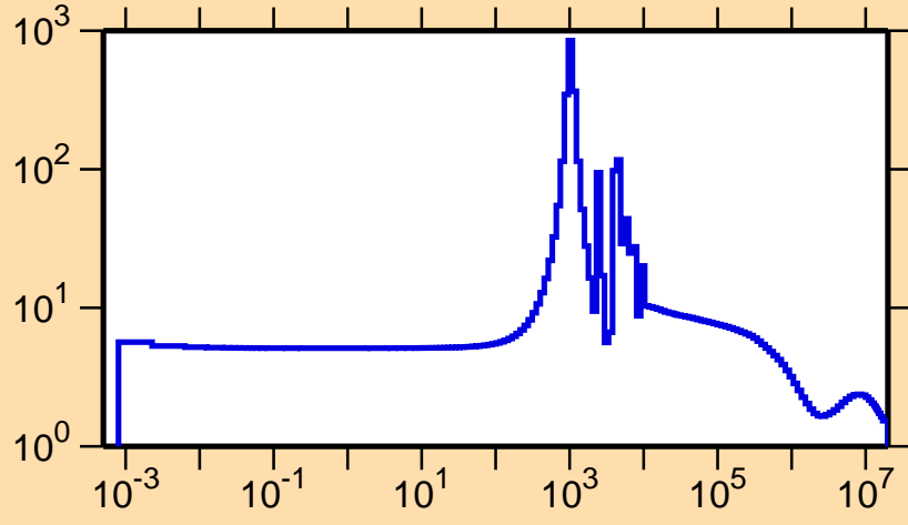
\sigma vs. E for ^{81}\text{As}(n,\text{el.})
