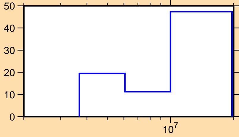
\Delta\sigma/\sigma vs. E for ^{81}\text{As}(n,n\text{cont.})
