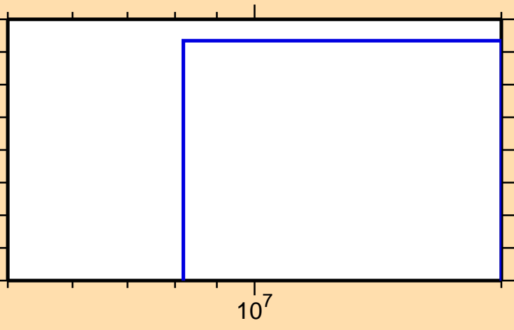
\sigma vs. E for ^{81}\text{As}(n,2np)
