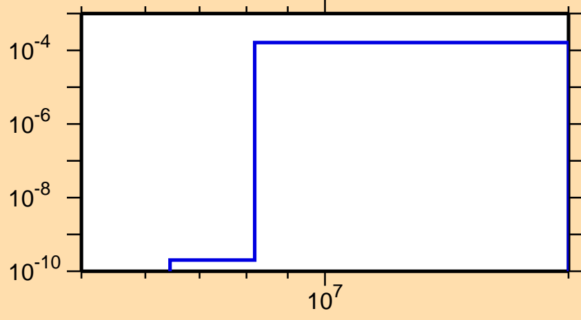
\sigma vs. E for ^{81}\text{As}(n,\alpha)
