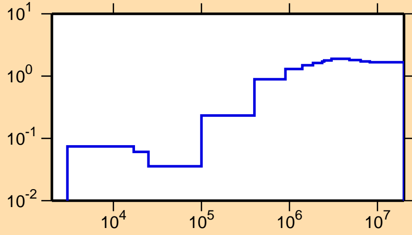
\sigma vs. E for ^{81}\text{As}(n,\text{nonel.})
