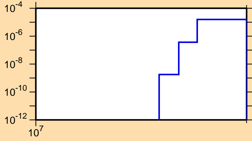
\sigma vs. E for ^{82}\text{As}(n,nd)
