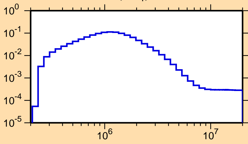
\sigma vs. E for ^{82}\text{As}(n,n_1)
