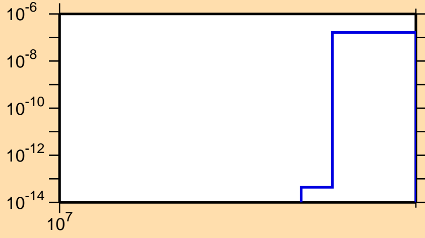
\sigma vs. E for ^{82}\text{As}(n,nt)
