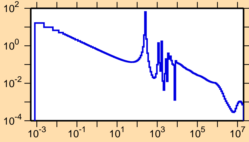
\sigma vs. E for ^{82}\text{As}(n,\gamma)
