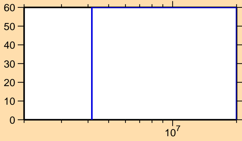
\Delta\sigma/\sigma vs. E for ^{82}\text{As}(n,\gamma)
