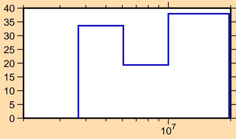
\Delta\sigma/\sigma vs. E for ^{82}\text{As}(n,el.)
