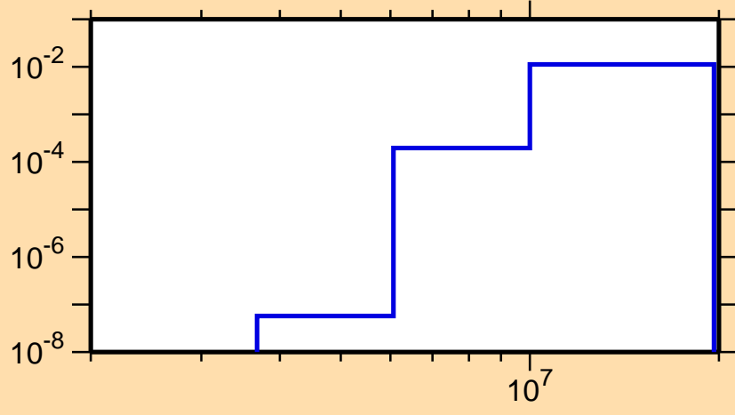
\sigma vs. E for ^{82}\text{As}(n,p)
