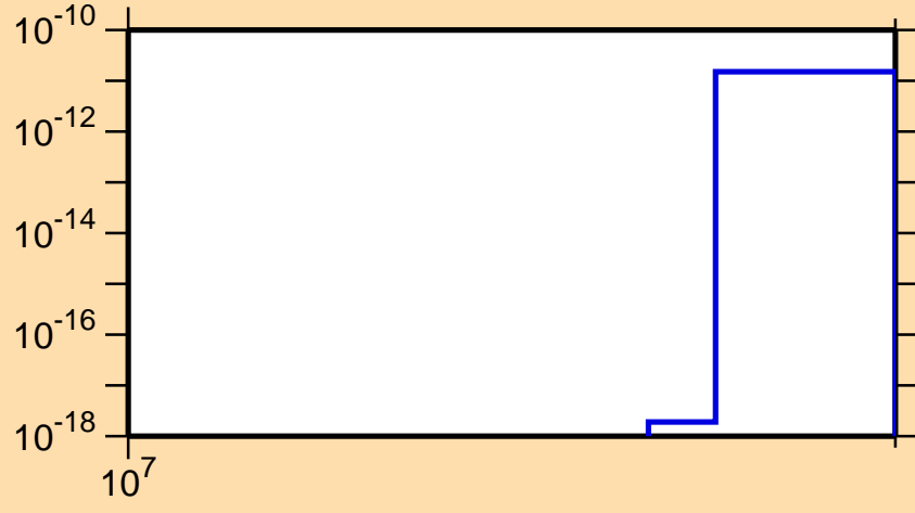
\sigma vs. E for ^{82}\text{As}(n,2n\alpha)
