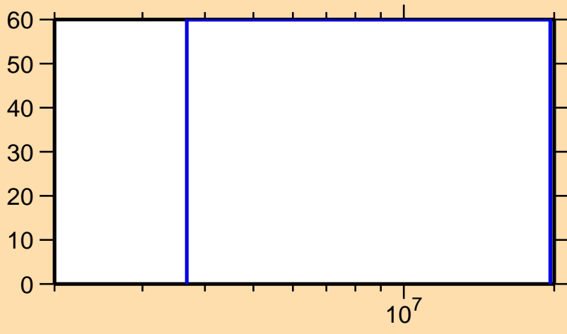
\Delta\sigma/\sigma vs. E for ^{82}\text{As}(n,p)
