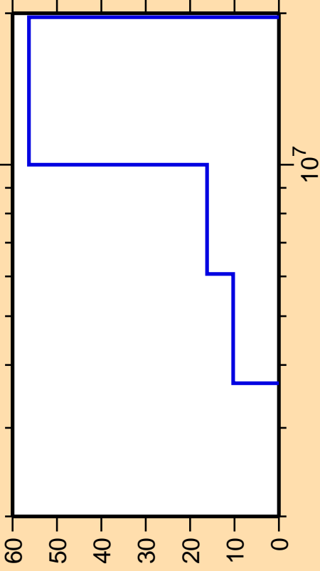
\Delta\sigma/\sigma vs. E for ^{82}\text{As}(n,n\text{cont.})
