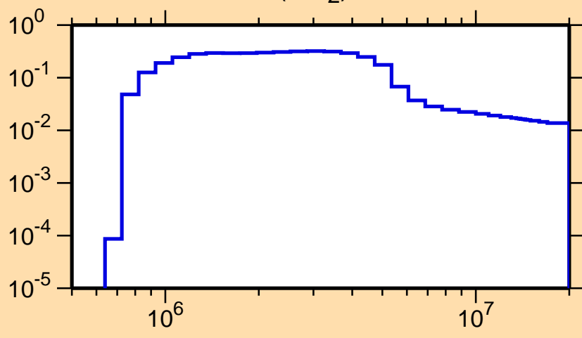
\sigma vs. E for ^{83}\text{As}(n,n_2)
