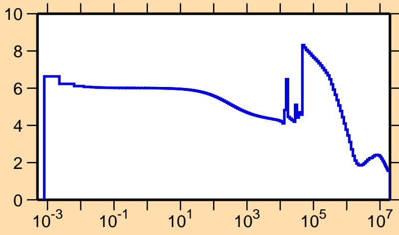
\sigma vs. E for ^{83}\text{As}(n,\text{el.})
