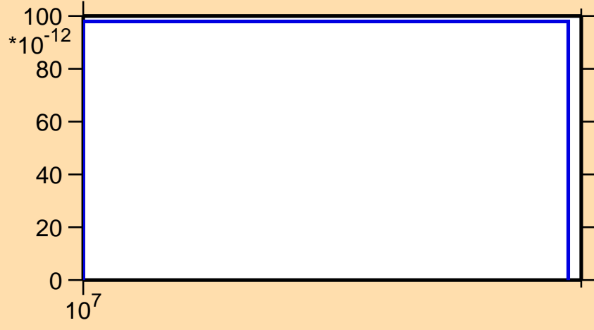
\sigma vs. E for ^{83}\text{As}(n,nd)
