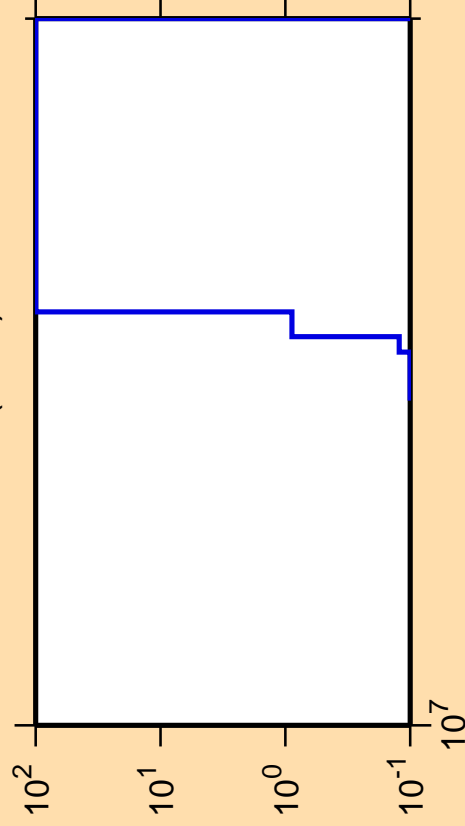
\Delta\sigma/\sigma vs. E for ^{84}\text{As}(n,nd)
