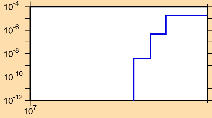
\sigma vs. E for ^{84}\text{As}(n,nd)
