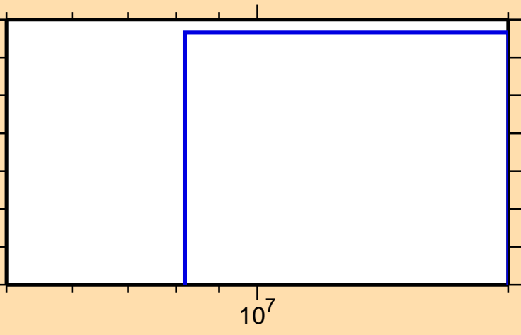
\sigma vs. E for ^{85}\text{As}(n,t)
