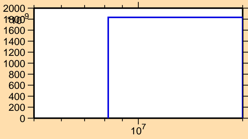
\sigma vs. E for ^{85}\text{As}(n,n\alpha)
