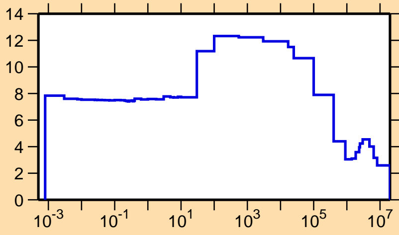
\sigma vs. E for ^{197}\text{At}(n,\text{el.})
