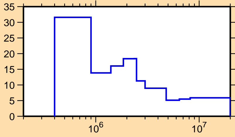
\Delta\sigma/\sigma vs. E for ^{197}\text{At}(n,\text{nonel.})
