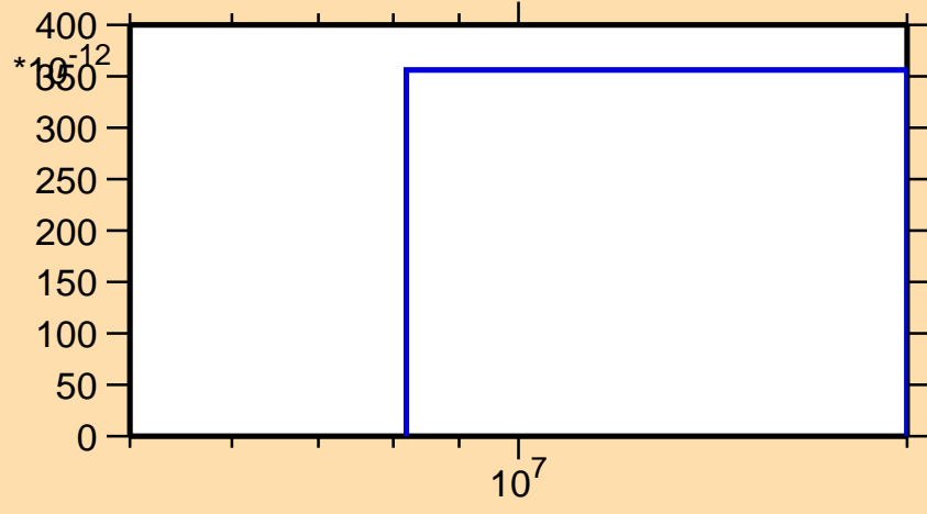
\sigma vs. E for ^{197}\text{At}(n,nt)
