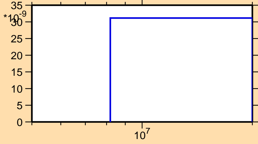
\sigma vs. E for ^{197}\text{At}(n,3n)
