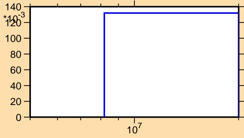
\sigma vs. E for ^{197}\text{At}(n,2n)
