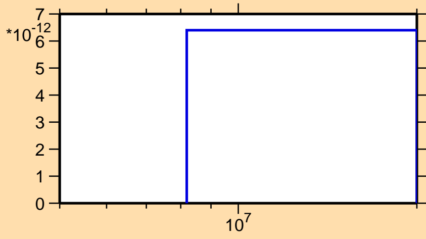
\sigma vs. E for ^{197}\text{At}(\text{mt } 34)
