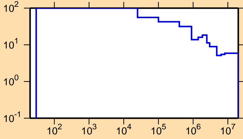
\Delta\sigma/\sigma vs. E for ^{197}\text{At}(n,\text{nonel.})
