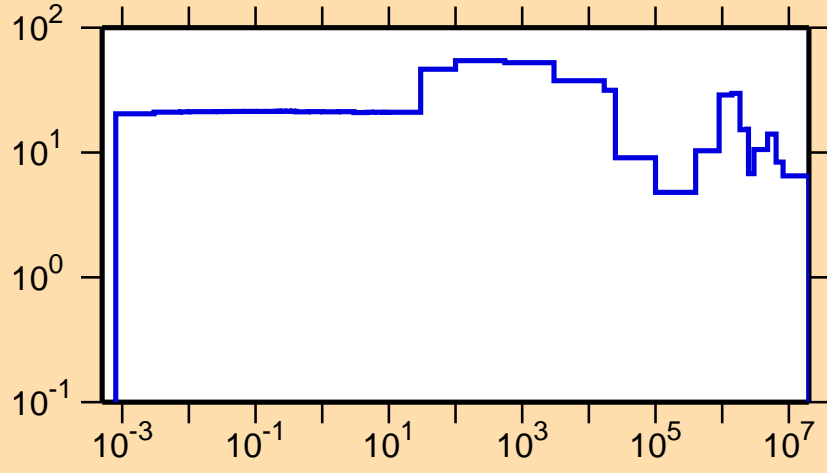
\Delta\sigma/\sigma vs. E for ^{197}\text{At}(n,\text{el.})
