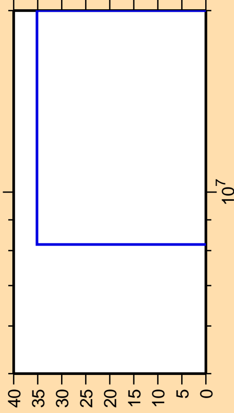
\Delta\sigma/\sigma vs. E for ^{197}\text{At}(\text{mt } 34)
