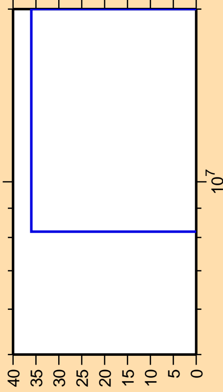
\Delta\sigma/\sigma vs. E for ^{197}\text{At}(n,n\text{cont.})
