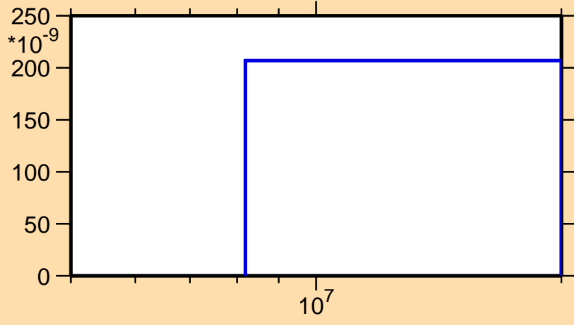
\sigma vs. E for ^{197}\text{At}(n,\text{pd})
