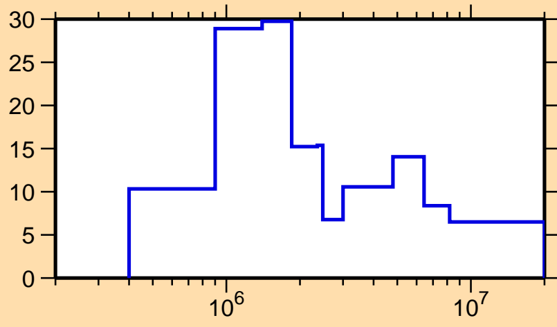
\Delta\sigma/\sigma vs. E for ^{197}\text{At}(n, el.)
