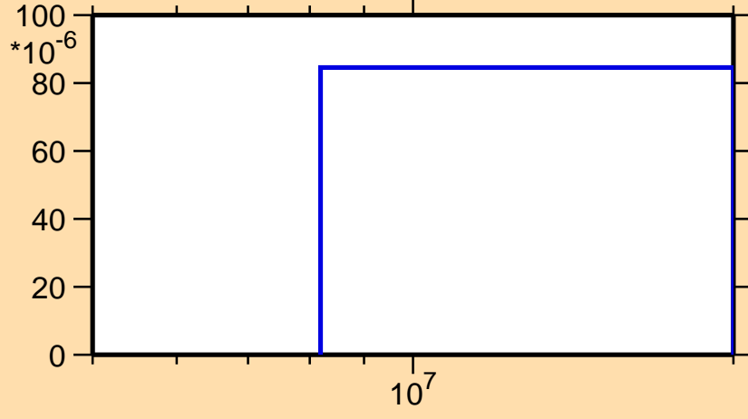
\sigma vs. E for ^{197}\text{At}(n,2np)
