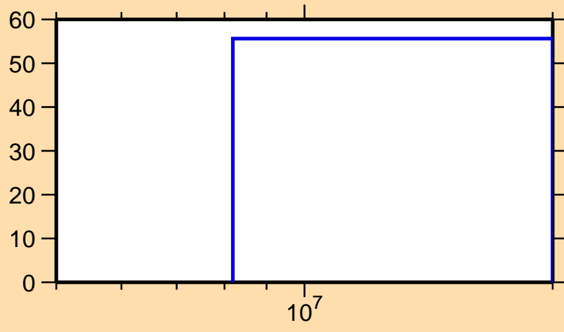
\Delta\sigma/\sigma vs. E for ^{197}\text{At}(n,2n)
