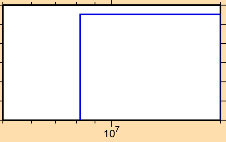
\sigma vs. E for ^{197}\text{At}(n,3n\alpha)
