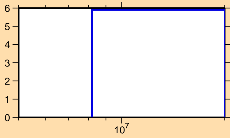
\Delta\sigma/\sigma vs. E for ^{197}\text{At}(n,\text{nonel.})
