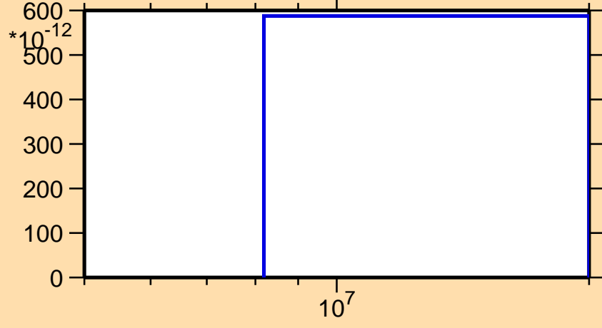
\sigma vs. E for ^{197}\text{At}(n,pt)
