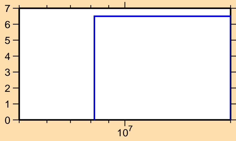
\Delta\sigma/\sigma vs. E for ^{197}\text{At}(n,\text{el.})
