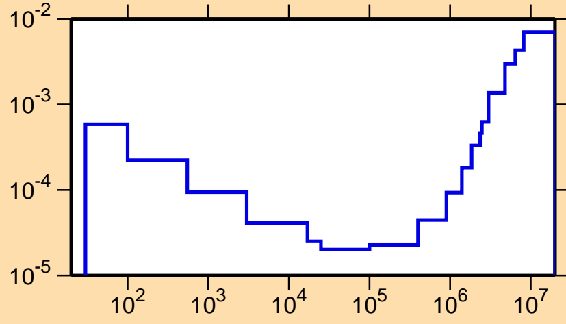
\sigma vs. E for ^{197}\text{At}(n,p\alpha)
