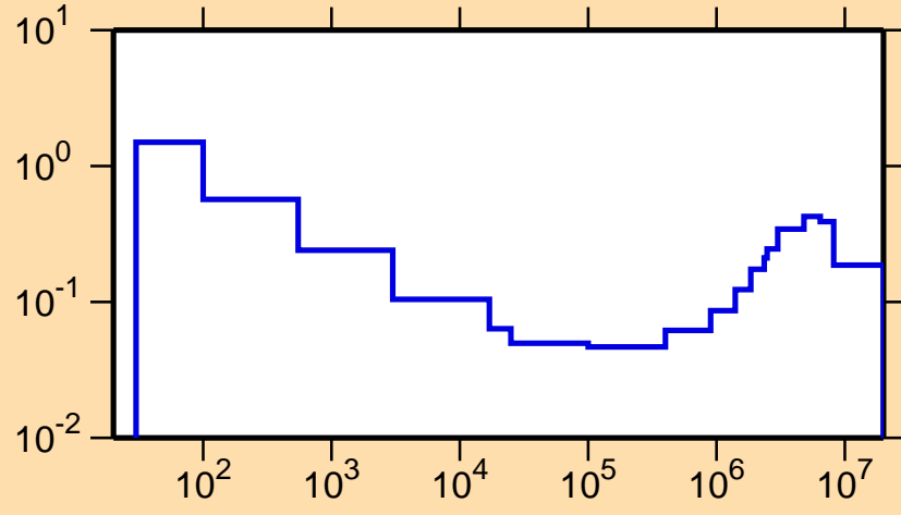
\sigma vs. E for ^{197}\text{At}(n,p)
