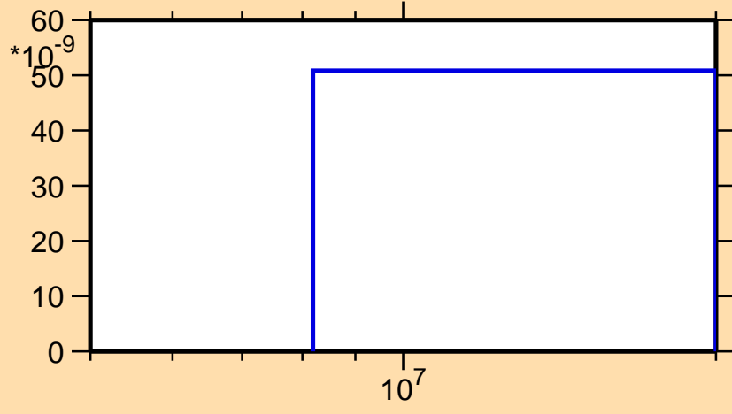
\sigma vs. E for ^{197}\text{At}(n,\text{nd})
