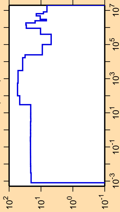
\Delta\sigma/\sigma vs. E for ^{197}\text{At}(n,\text{el.})
