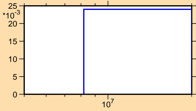
\sigma vs. E for ^{197}\text{At}(n,2n\alpha)
