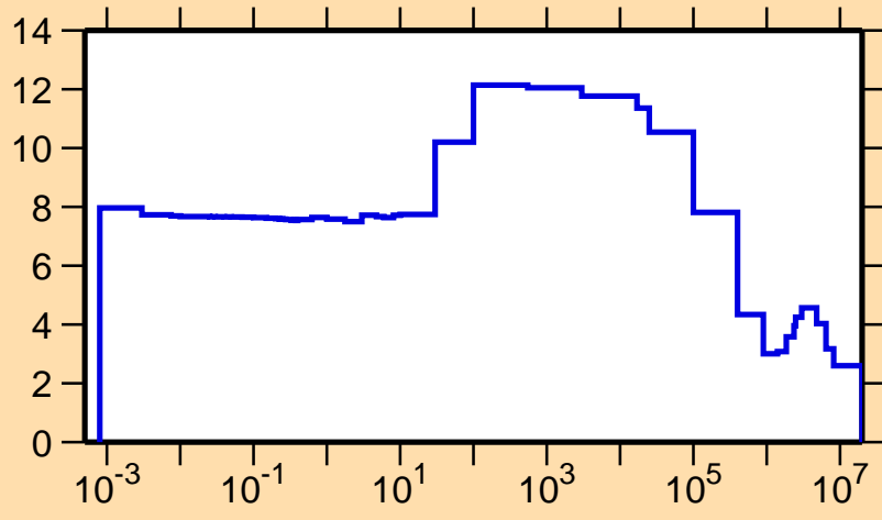
\sigma vs. E for ^{198}\text{At}(n,\text{el.})
