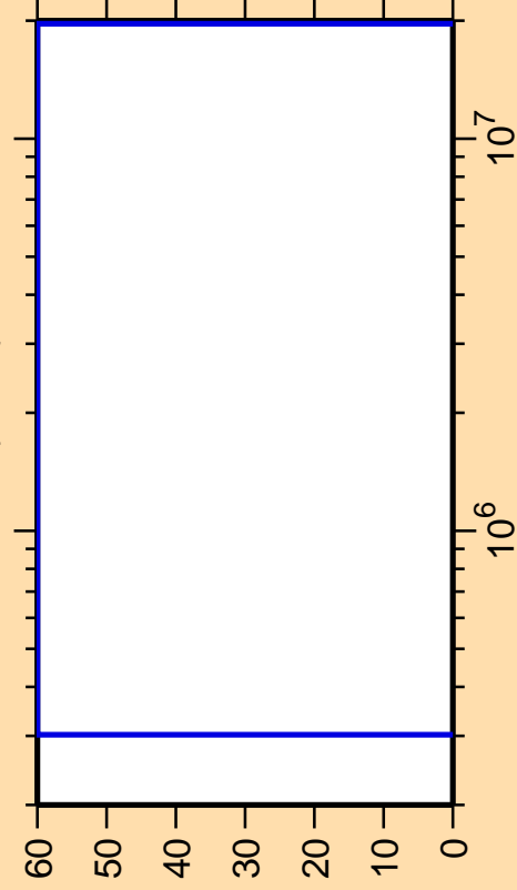
\Delta\sigma/\sigma vs. E for ^{200}\text{At}(n,n\alpha)
