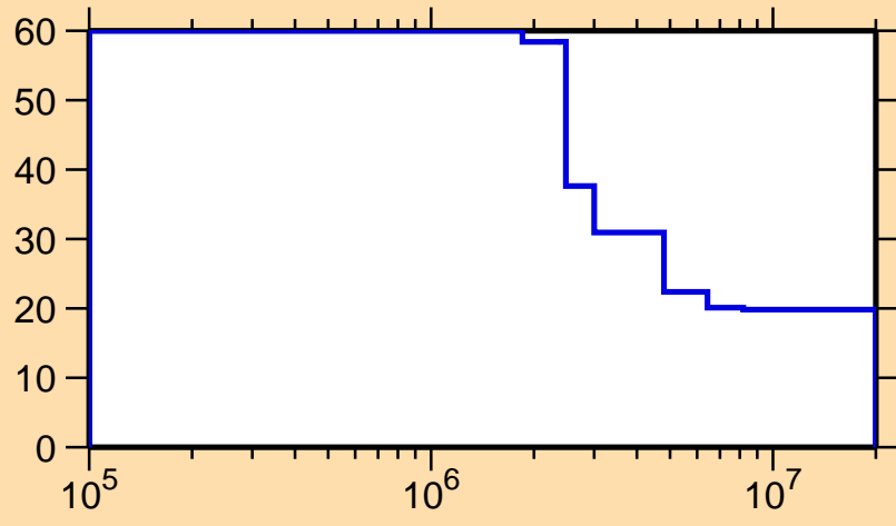
\Delta\sigma/\sigma vs. E for ^{200}\text{At}(n,n\text{cont.})
