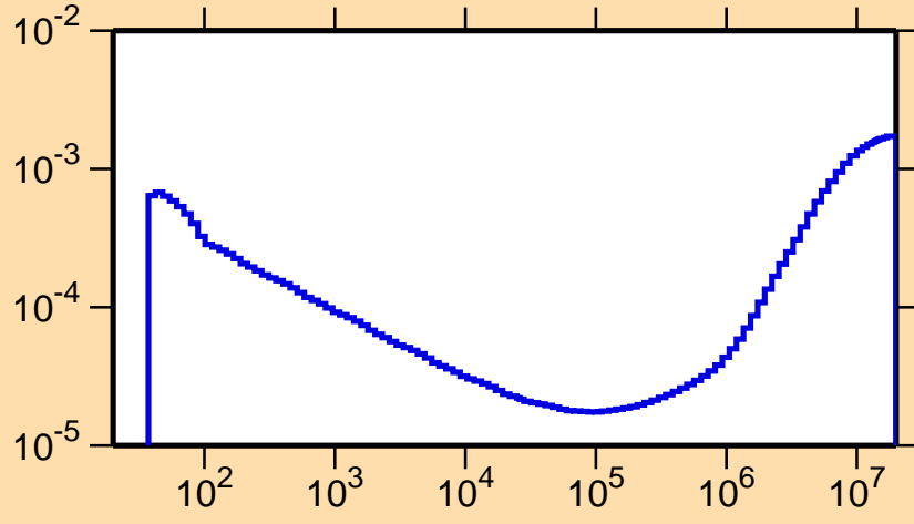
\sigma vs. E for ^{200}\text{At}(n,p\alpha)
