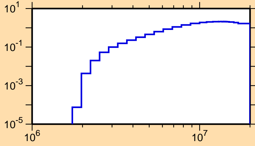
\sigma vs. E for ^{201}\text{At}(n,n\text{cont.})
