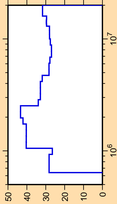
\Delta\sigma/\sigma vs. E for ^{201}\text{At}(n,n_1)
