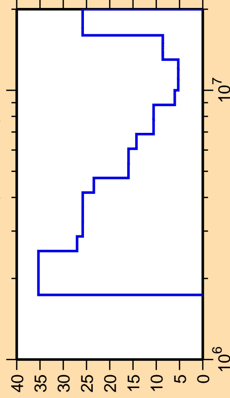
\Delta\sigma/\sigma vs. E for ^{201}\text{At}(n,n\text{cont.})
