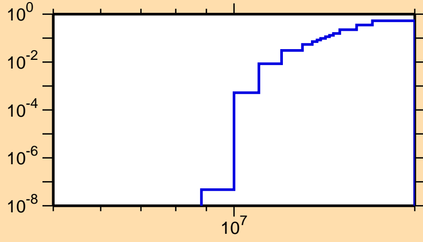
\sigma vs. E for ^{201}\text{At}(n,2n)
