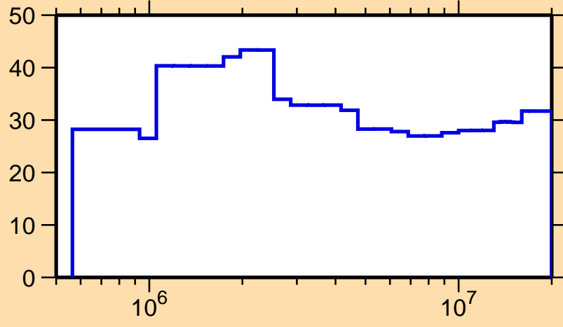
\Delta\sigma/\sigma vs. E for ^{201}\text{At}(n,n_1)
