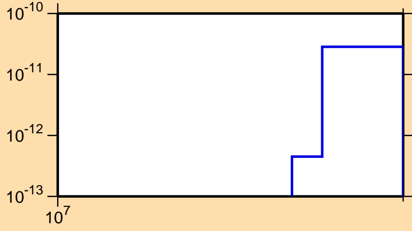
\sigma vs. E for ^{201}\text{At}(n,pt)
