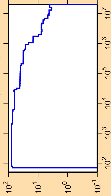
\Delta\sigma/\sigma vs. E for ^{201}\text{At}(n,\text{nonel.})
