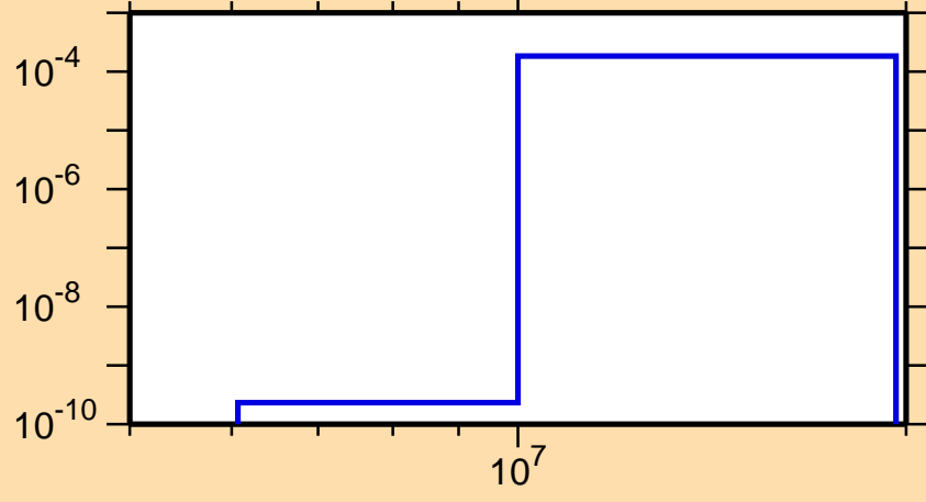
\sigma vs. E for ^{201}\text{At}(n,t)
