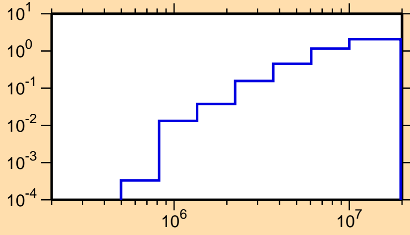
\sigma vs. E for ^{201}\text{At}(n,\text{inel.})
