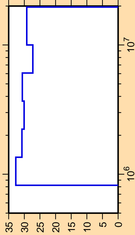
\Delta\sigma/\sigma vs. E for ^{201}\text{At}(n,n_3)
