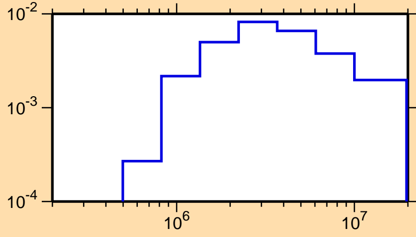
\sigma vs. E for ^{201}\text{At}(n,n_1)
