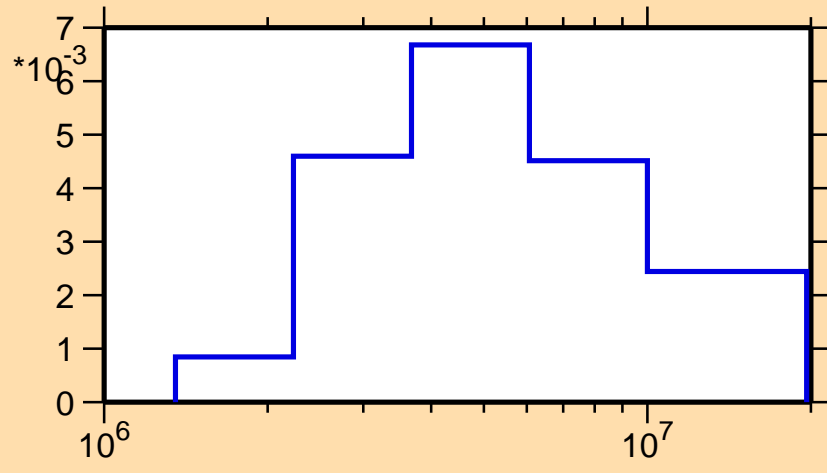
\sigma vs. E for ^{201}\text{At}(n,n_4)
