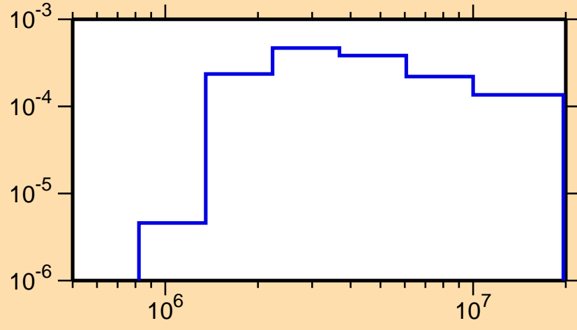
\sigma vs. E for ^{201}\text{At}(n,n_3)
