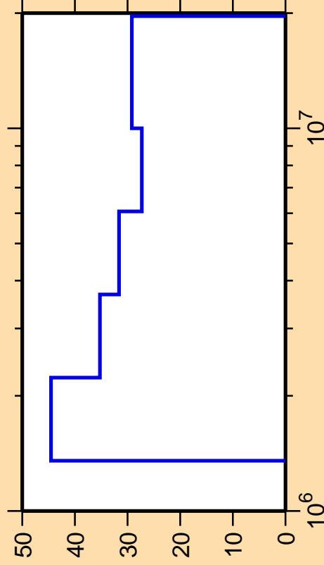
\Delta\sigma/\sigma vs. E for ^{201}\text{At}(n,n_4)
