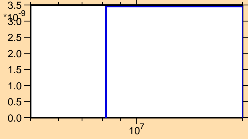
\sigma vs. E for ^{201}\text{At}(n,\text{nd})
