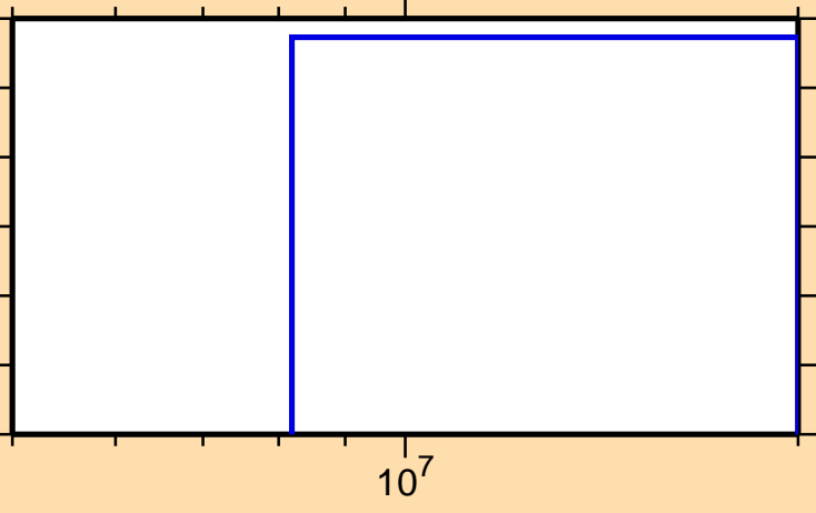
\sigma vs. E for ^{201}\text{At}(n,\text{pd})
