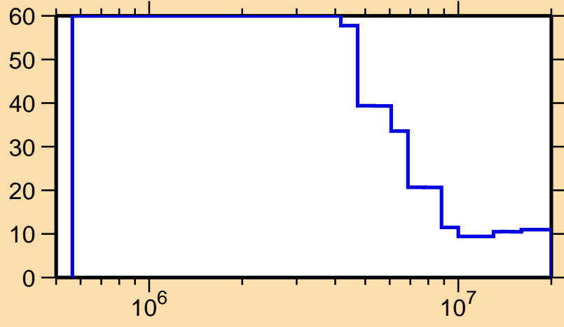
\Delta\sigma/\sigma vs. E for ^{202}\text{At}(n,n\text{cont.})
