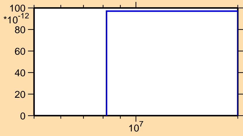
\sigma vs. E for ^{202}\text{At}(n,3n\alpha)
