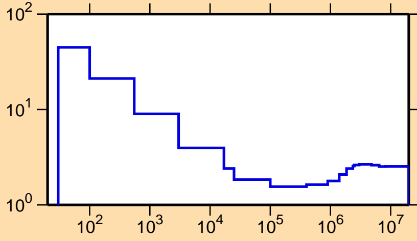
\sigma vs. E for ^{202}\text{At}(n,\text{nonel.})
