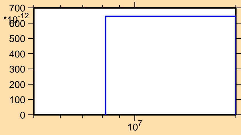
\sigma vs. E for ^{202}\text{At}(n,\text{pd})
