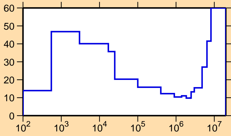
\Delta\sigma/\sigma vs. E for ^{202}\text{At}(n,\gamma)
