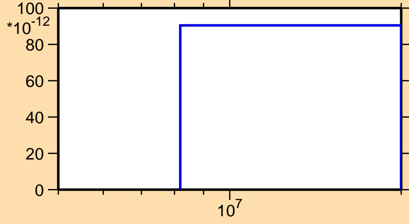
\sigma vs. E for ^{202}\text{At}(n,3n\alpha)
