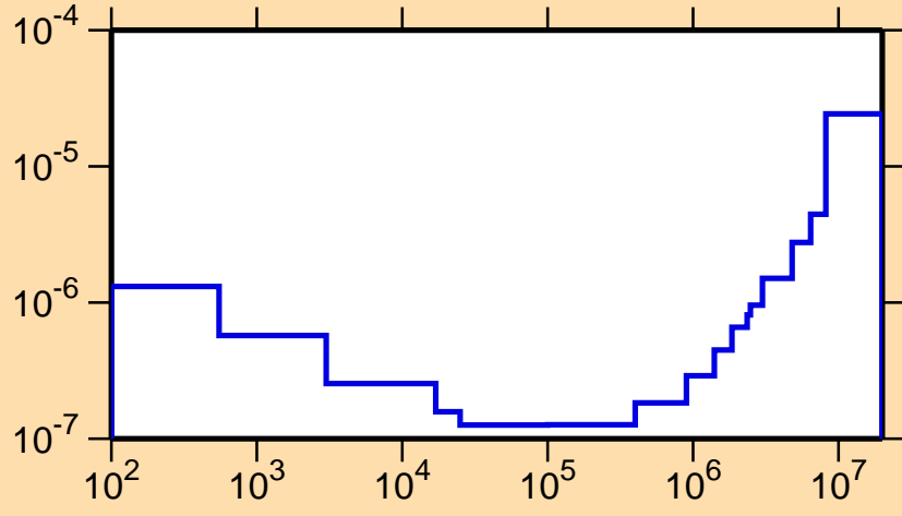
\sigma vs. E for ^{202}\text{At}(n,p\alpha)
