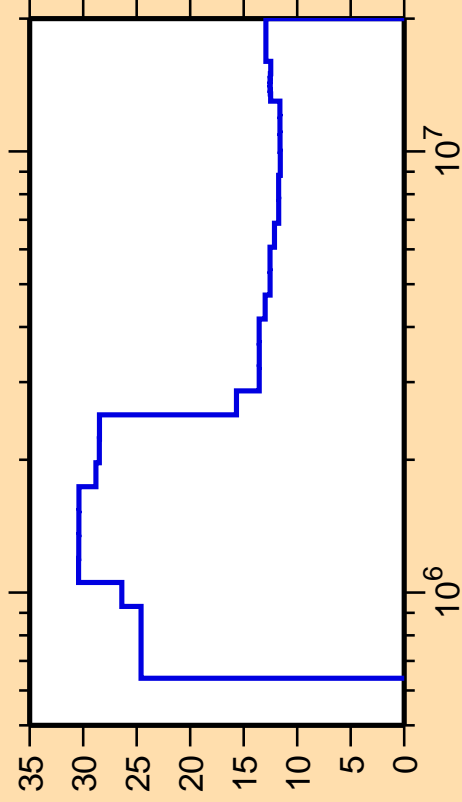
\Delta\sigma/\sigma vs. E for ^{203}\text{At}(n,n_2)
