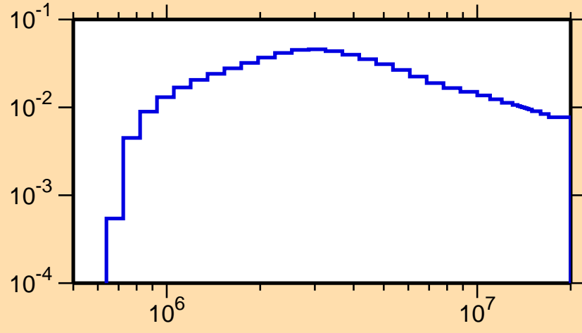
\sigma vs. E for ^{203}\text{At}(n,n_2)
