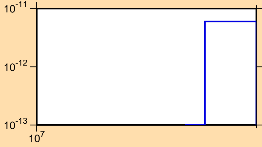
\sigma vs. E for ^{203}\text{At}(\text{mt } 34)
