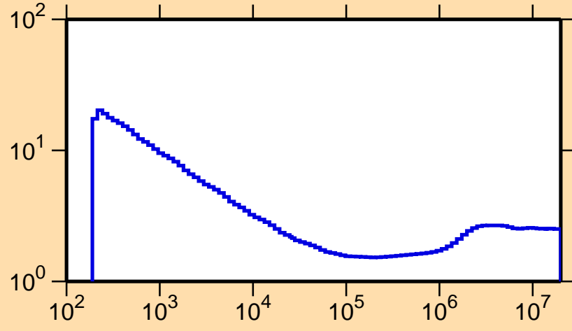
\sigma vs. E for ^{203}\text{At}(n,\text{nonel.})
