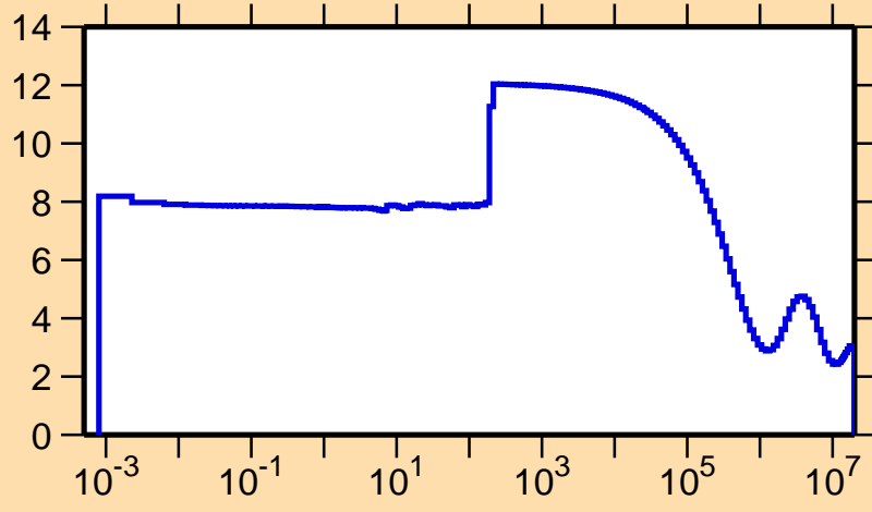
\sigma vs. E for ^{203}\text{At}(n,\text{el.})
