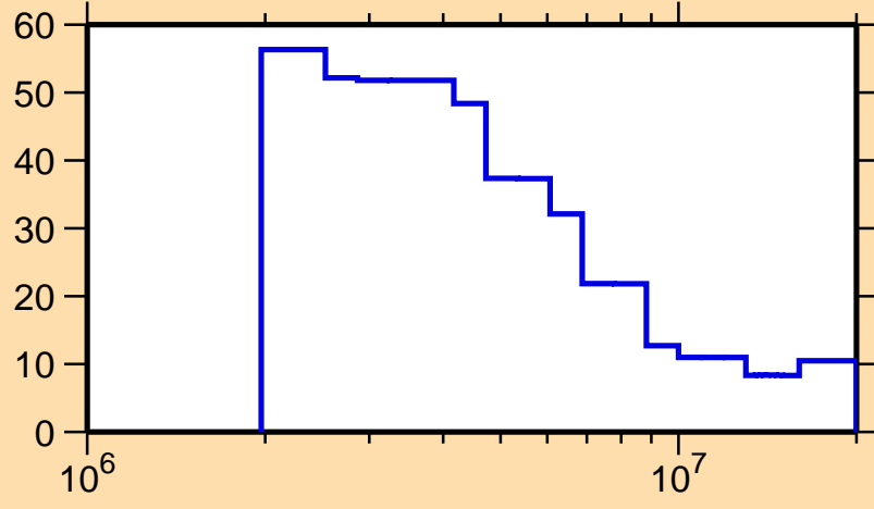
\Delta\sigma/\sigma vs. E for ^{203}\text{At}(n,n\text{cont.})
