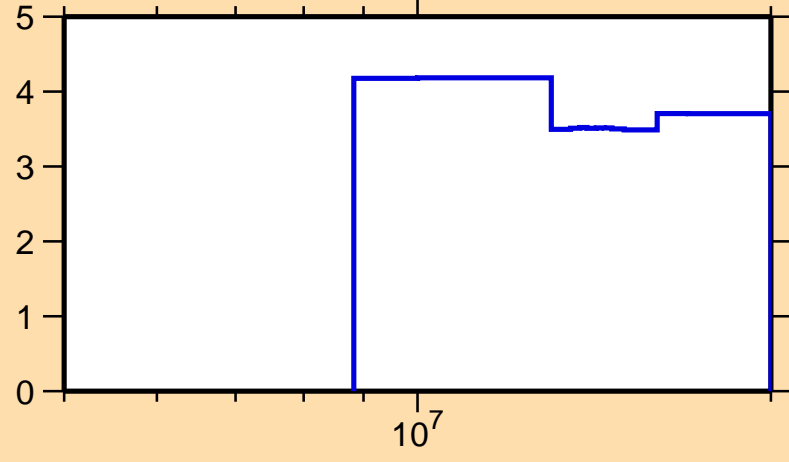
\Delta\sigma/\sigma vs. E for ^{203}\text{At}(n,\text{nonel.})
