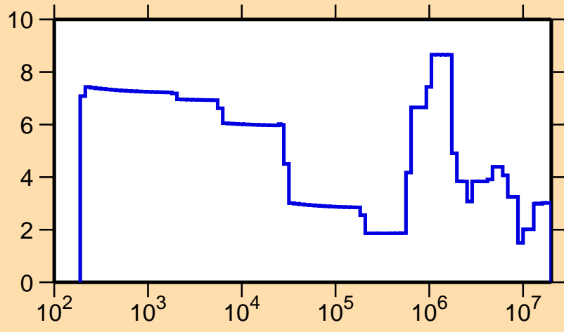
\Delta\sigma/\sigma vs. E for ^{203}\text{At}(n, \text{el.})
