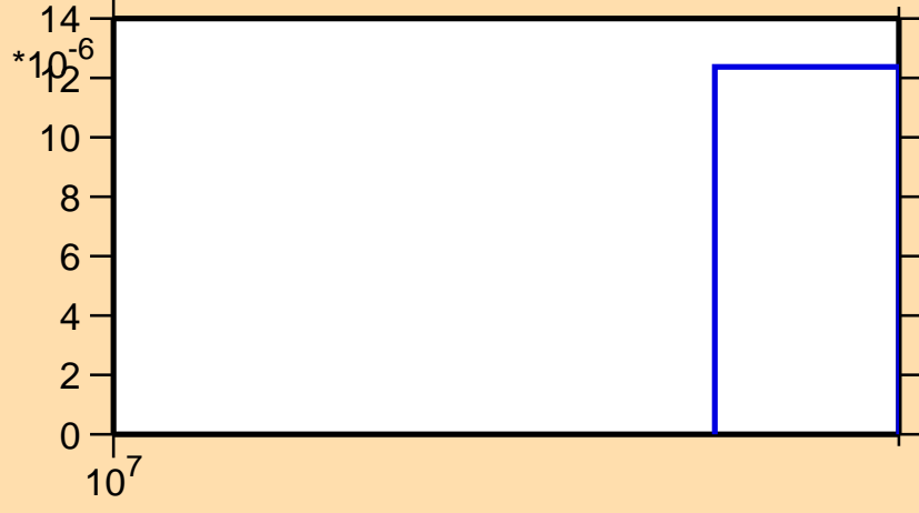
\sigma vs. E for ^{203}\text{At}(n,3n)
