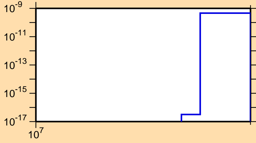
\sigma vs. E for ^{203}\text{At}(n,3n\alpha)
