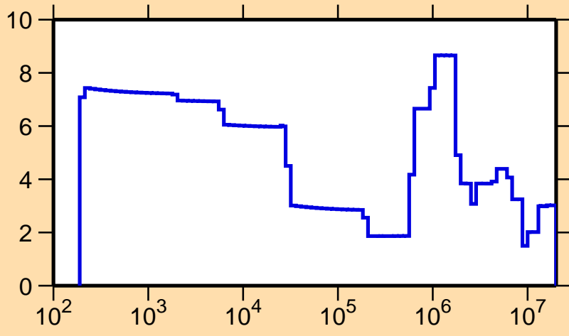
\Delta\sigma/\sigma vs. E for ^{203}\text{At}(n,el.)
