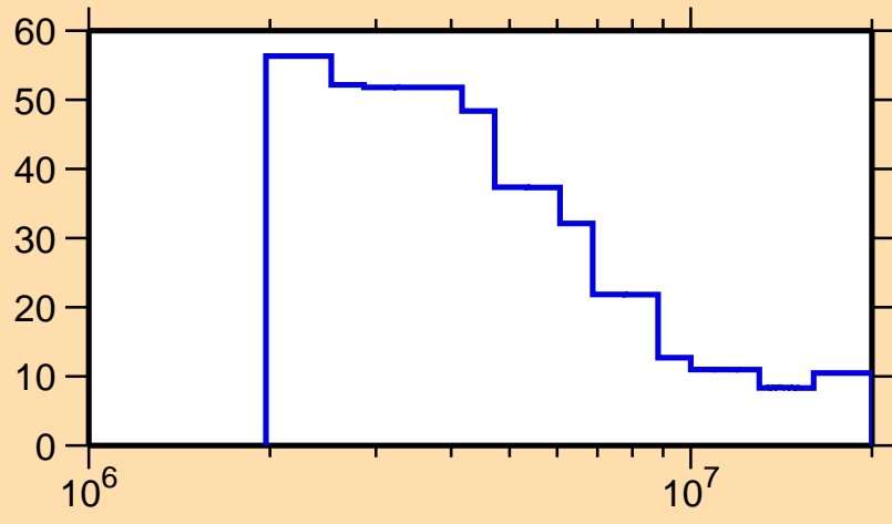
\Delta\sigma/\sigma vs. E for ^{203}\text{At}(n, ncont.)
