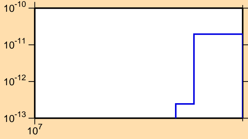
\sigma vs. E for ^{203}\text{At}(n,pt)
