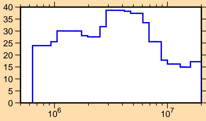
\Delta\sigma/\sigma vs. E for ^{203}\text{At}(n,\text{inel.})
