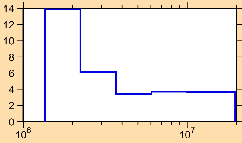
\Delta\sigma/\sigma vs. E for ^{203}\text{At}(n,n\text{nonel.})
