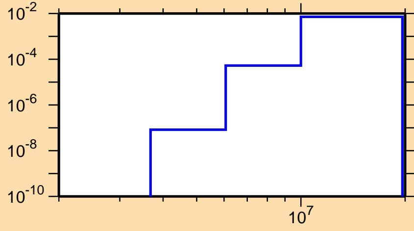
\sigma vs. E for ^{203}\text{At}(n,np)
