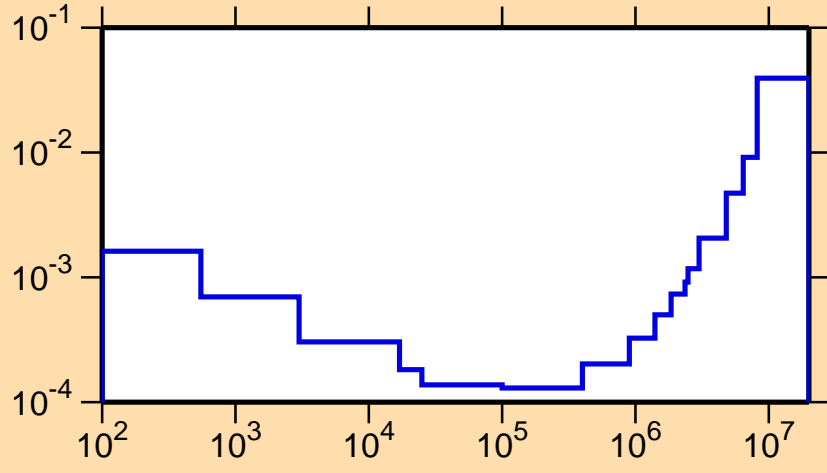
\sigma vs. E for ^{203}\text{At}(n,p)
