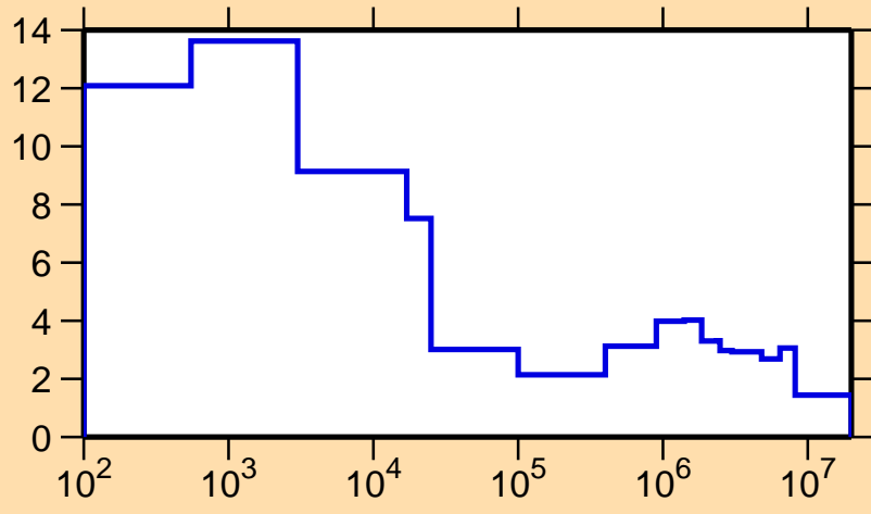
\Delta\sigma/\sigma vs. E for ^{203}\text{At}(n,\text{tot.})
