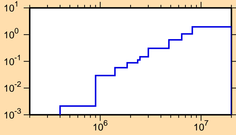
\sigma vs. E for ^{203}\text{At}(n,\text{inel.})
