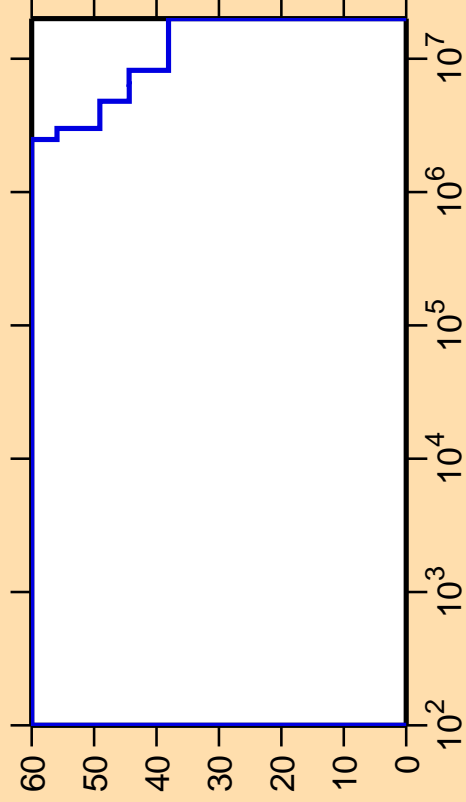
\Delta\sigma/\sigma vs. E for ^{203}\text{At}(n,p)
