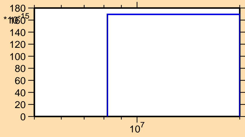
\sigma vs. E for ^{203}\text{At}(n,\text{pt})
