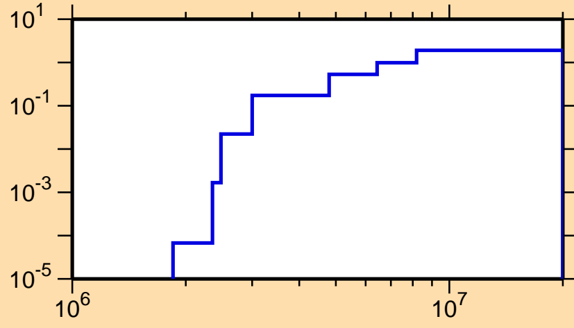
\sigma vs. E for ^{203}\text{At}(n,n\text{cont.})
