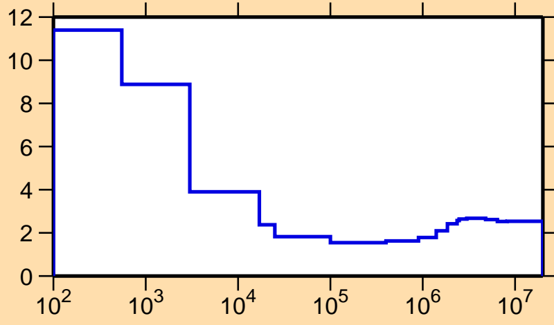
\sigma vs. E for ^{203}\text{At}(n,\text{nonel.})
