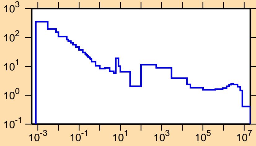
\sigma vs. E for ^{203}\text{At}(n,\gamma)
