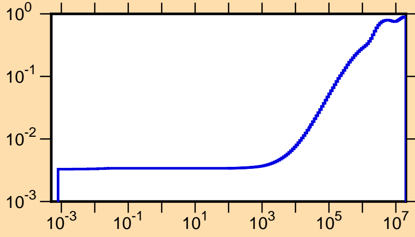
\mu vs. E for ^{205}\text{At}(\text{mt251})
