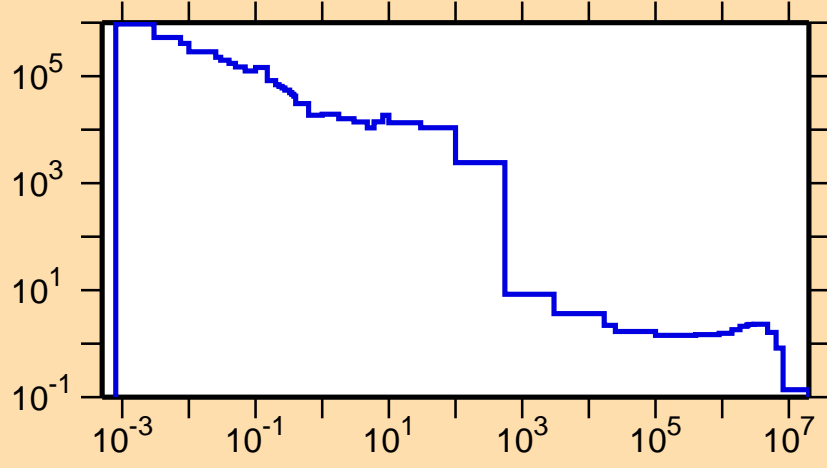
\sigma vs. E for ^{205}\text{At}(n,\gamma)
