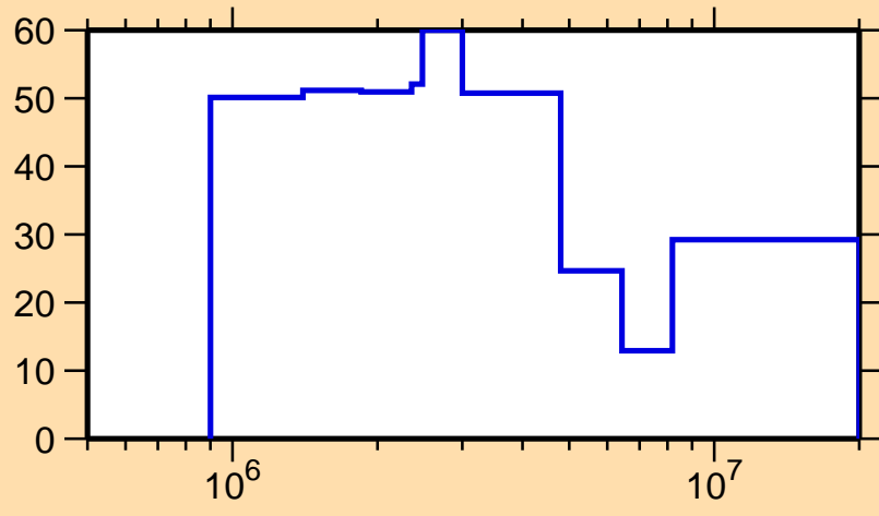
\Delta\sigma/\sigma vs. E for ^{205}\text{At}(n,ncont.)
