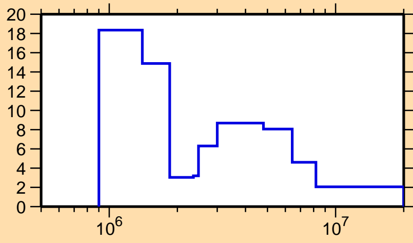
\Delta\sigma/\sigma vs. E for ^{205}\text{At}(n,\text{tot.})
