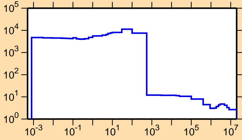
\sigma vs. E for ^{205}\text{At}(n,\text{el.})
