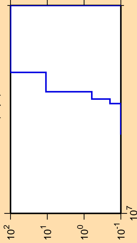
\Delta\sigma/\sigma vs. E for ^{206}\text{At}(n,pt)
