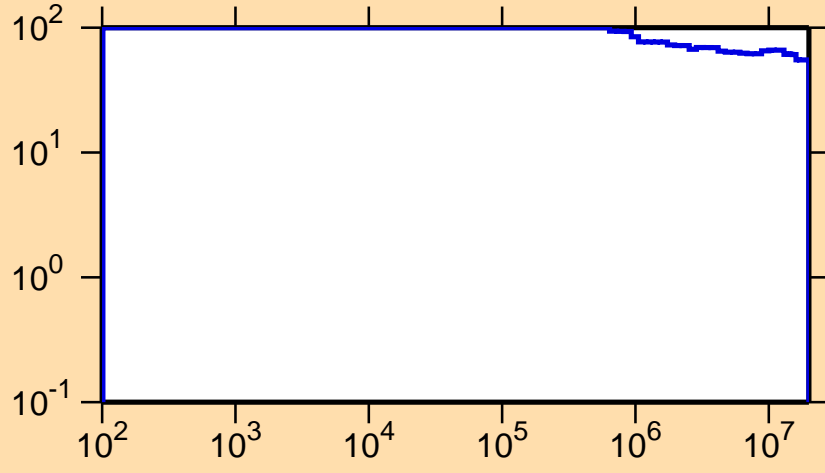
\Delta\sigma/\sigma vs. E for ^{206}\text{At}(n,p)
