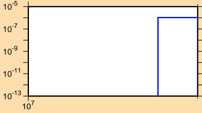
\sigma vs. E for ^{206}\text{At}(n,3n\alpha)
