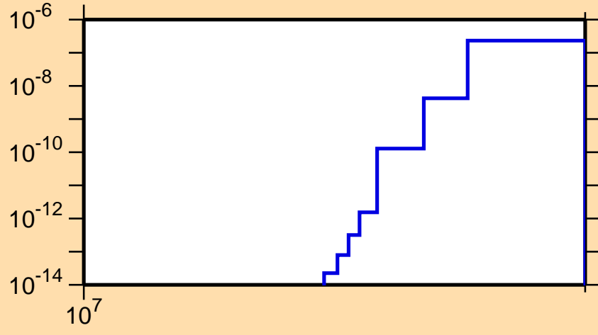
\sigma vs. E for ^{206}\text{At}(n,nt)
