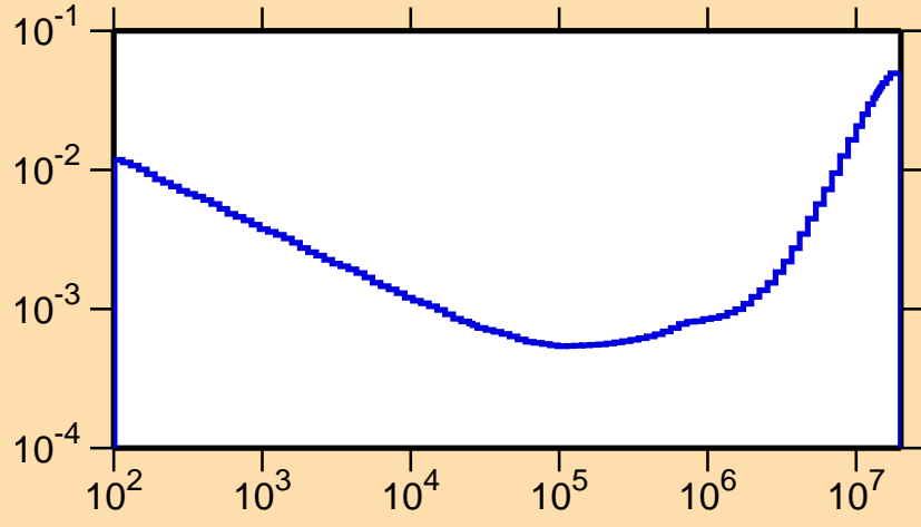
\sigma vs. E for ^{206}\text{At}(n,p)
