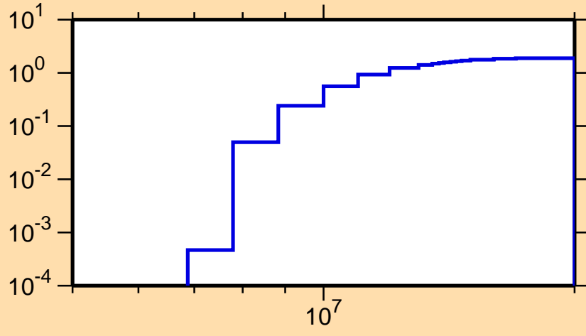
\sigma vs. E for ^{206}\text{At}(n,2n)
