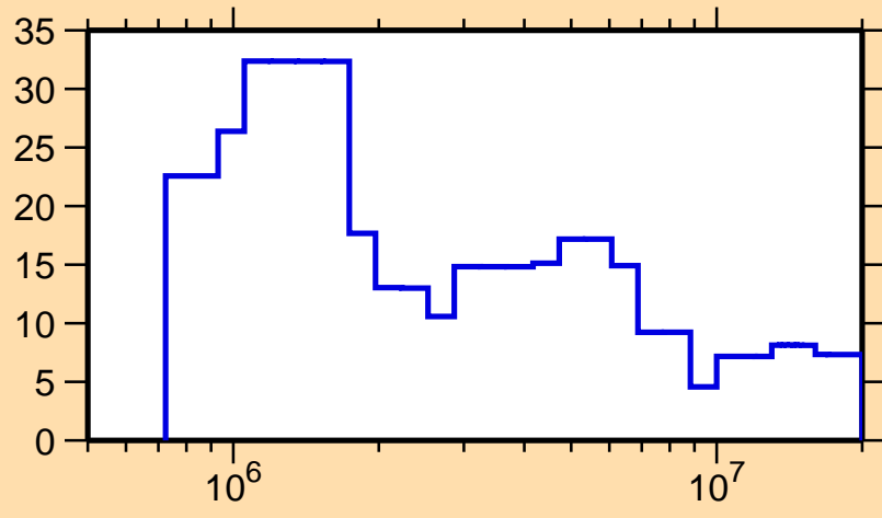
\Delta\sigma/\sigma vs. E for ^{206}\text{At}(n, el.)
