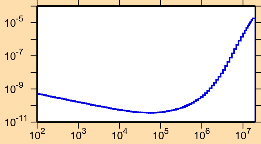
\sigma vs. E for ^{206}\text{At}(n,p\alpha)
