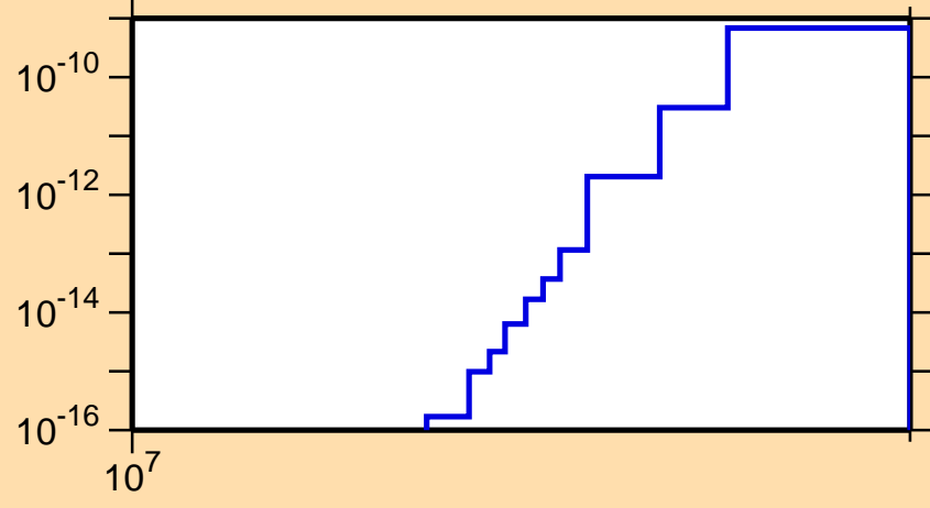
\sigma vs. E for ^{206}\text{At}(n,pt)
