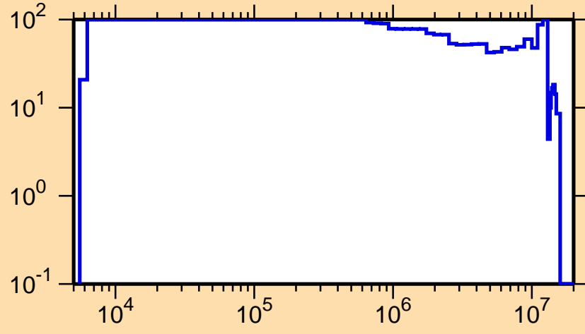
\Delta\sigma/\sigma vs. E for ^{206}\text{At}(n,n_1)
