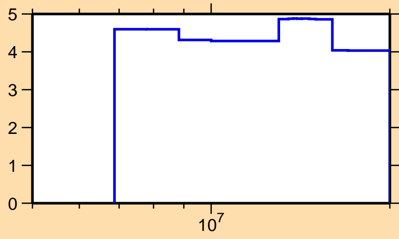
\Delta\sigma/\sigma vs. E for ^{206}\text{At}(n,\text{nonel.})
