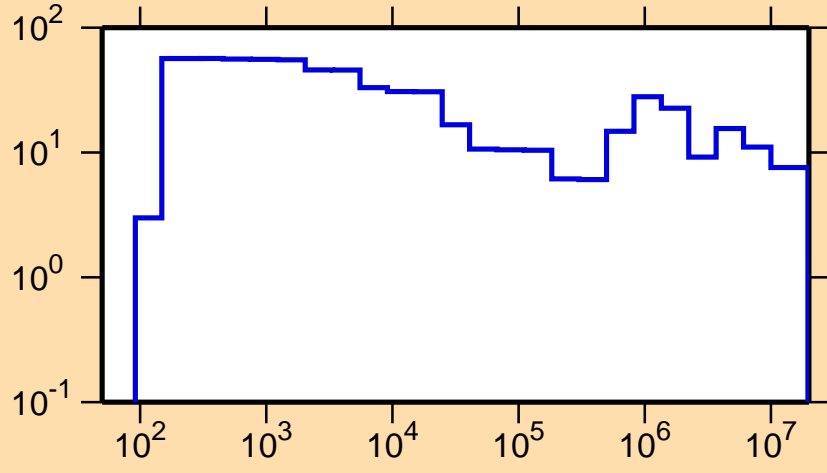
\Delta\sigma/\sigma vs. E for ^{206}\text{At}(n,el.)
