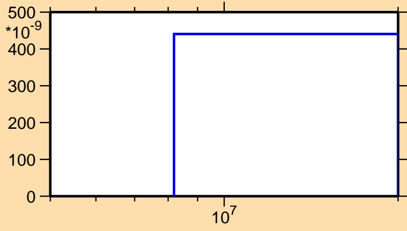
\sigma vs. E for ^{206}\text{At}(n,\text{nd})
