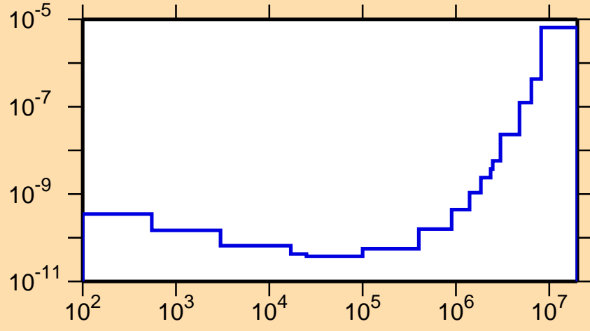
\sigma vs. E for ^{206}\text{At}(n,p\alpha)
