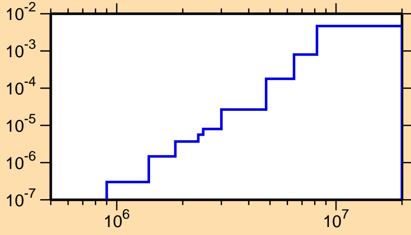
\sigma vs. E for ^{206}\text{At}(n,n\alpha)
