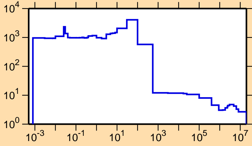
\sigma vs. E for ^{206}\text{At}(n,\text{el.})
