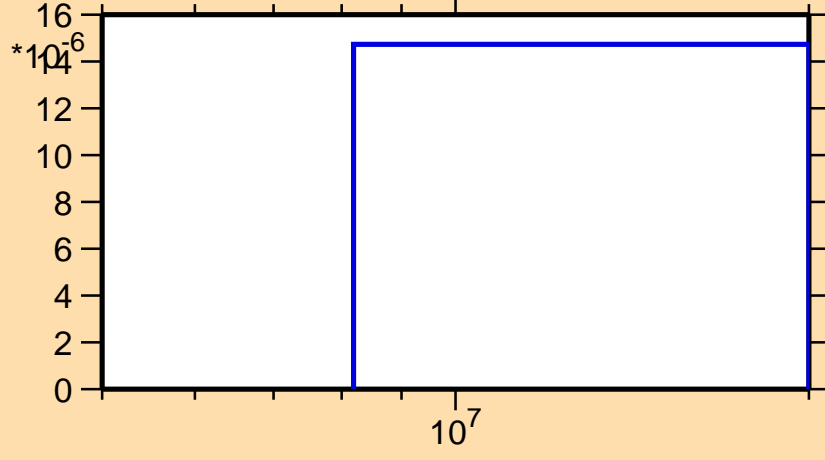
\sigma vs. E for ^{206}\text{At}(n,3n)
