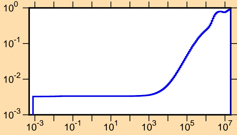
\mu vs. E for ^{207}\text{At}(\text{mt251})
