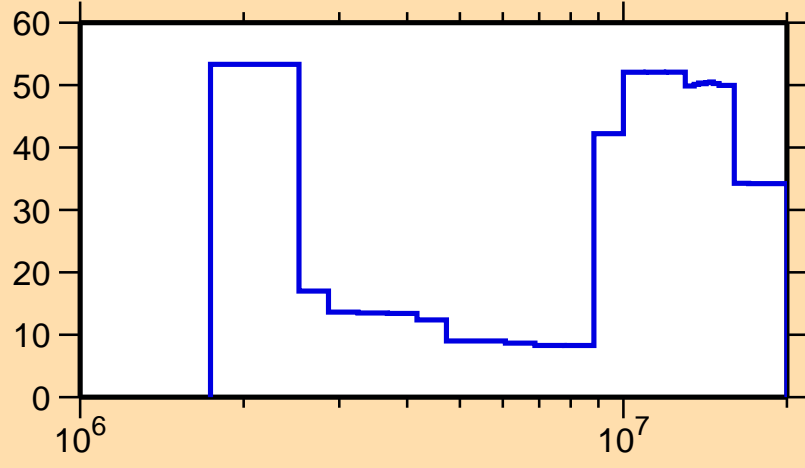
\Delta\sigma/\sigma vs. E for ^{207}\text{At}(n,n\text{cont.})
