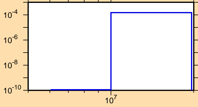
\sigma vs. E for ^{207}\text{At}(n,t)
