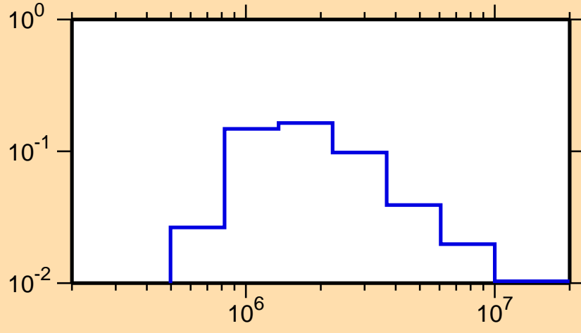
\sigma vs. E for ^{207}\text{At}(n,n_2)
