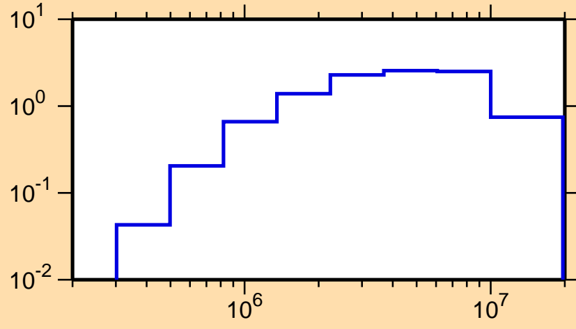
\sigma vs. E for ^{207}\text{At}(n,\text{inel.})
