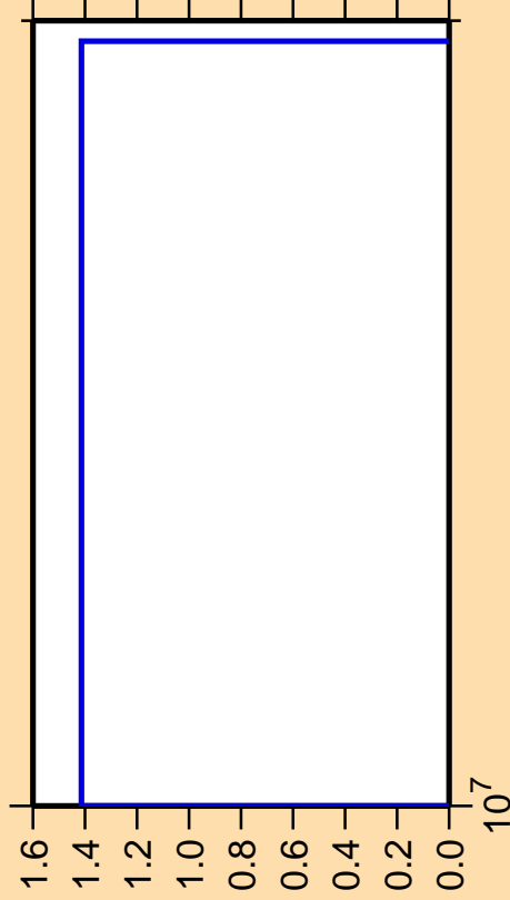
\Delta\sigma/\sigma vs. E for ^{207}\text{At}(n,\text{pt})
