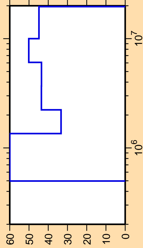
\Delta\sigma/\sigma vs. E for ^{207}\text{At}(n,n_2)
