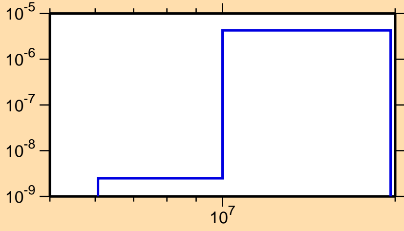
\sigma vs. E for ^{207}\text{At}(\text{mt117})
