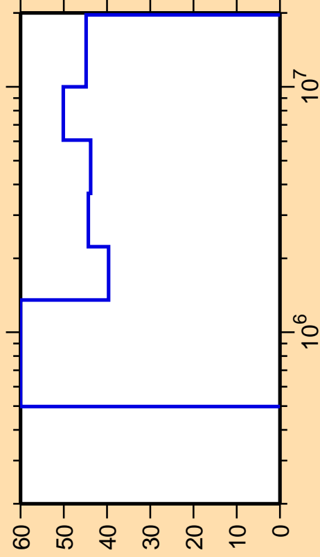
\Delta\sigma/\sigma vs. E for ^{207}\text{At}(n,n_4)
