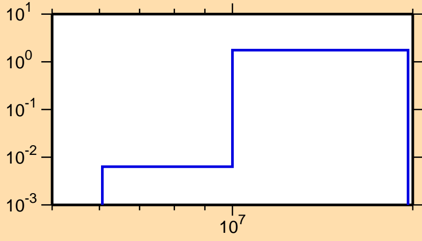
\sigma vs. E for ^{207}\text{At}(n,2n)
