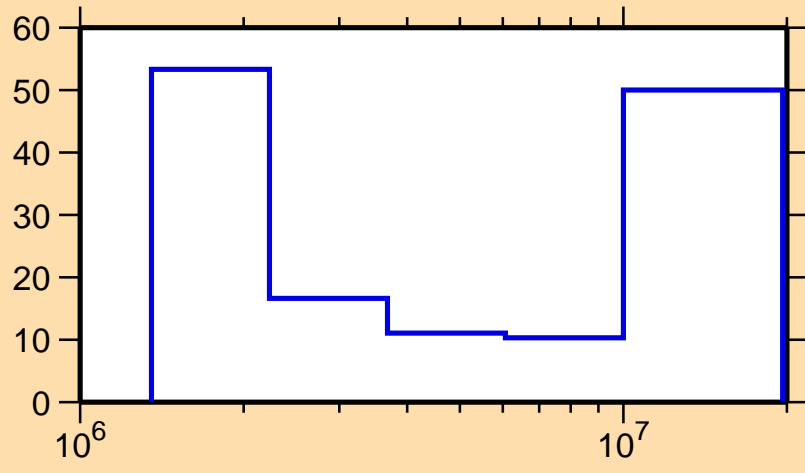
\Delta\sigma/\sigma vs. E for ^{207}\text{At}(n,n\text{cont.})
