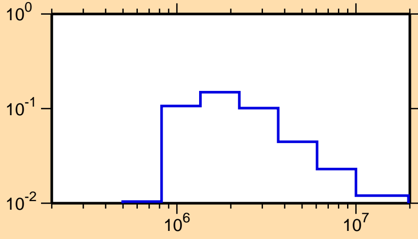
\sigma vs. E for ^{207}\text{At}(n,n_4)
