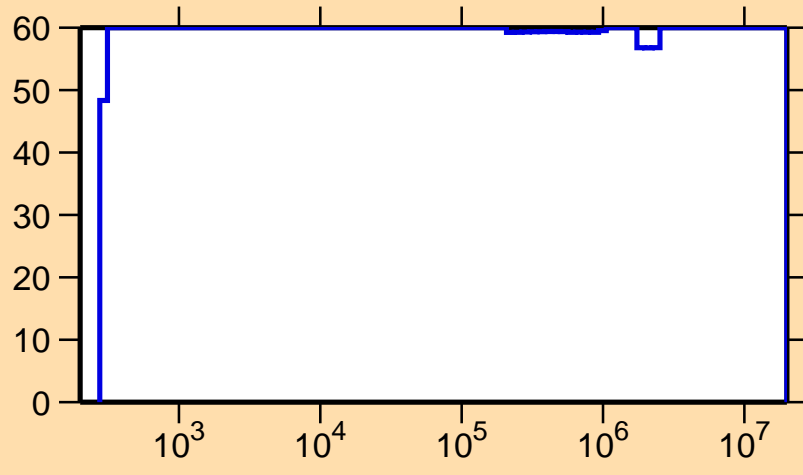
\Delta\sigma/\sigma vs. E for ^{208}\text{At}(n,\gamma)
