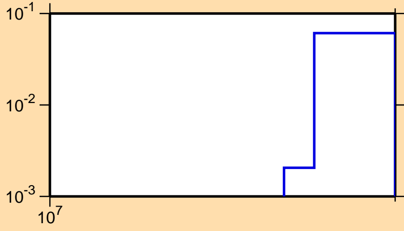
\sigma vs. E for ^{208}\text{At}(n,3n)
