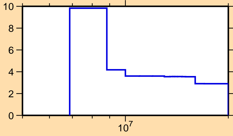
\Delta\sigma/\sigma vs. E for ^{208}\text{At}(n,\text{tot.})
