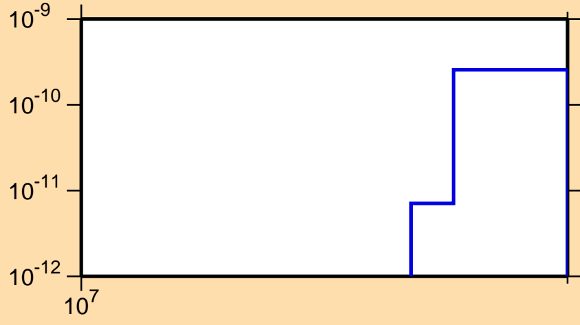
\sigma vs. E for ^{208}\text{At}(\text{mt } 34)
