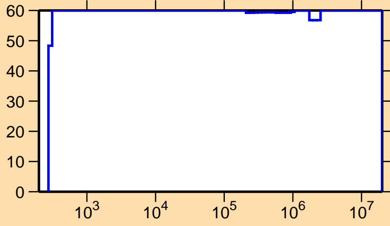
\Delta\sigma/\sigma vs. E for ^{208}\text{At}(n,\gamma)
