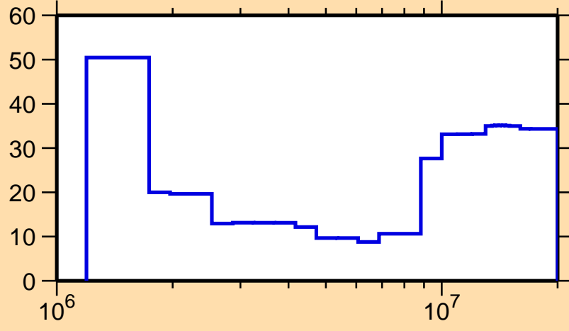
\Delta\sigma/\sigma vs. E for ^{208}\text{At}(n, ncont.)
