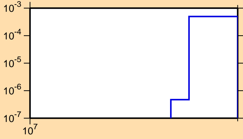
\sigma vs. E for ^{208}\text{At}(n,3n\alpha)
