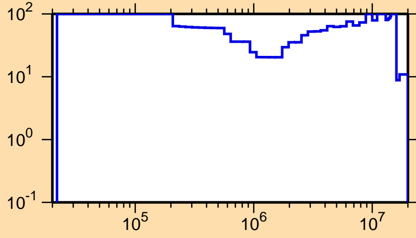
\Delta\sigma/\sigma vs. E for ^{208}\text{At}(n,n_1)
