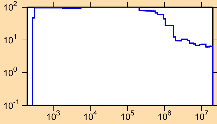
\Delta\sigma/\sigma vs. E for ^{208}\text{At}(n,\text{nonel.})
