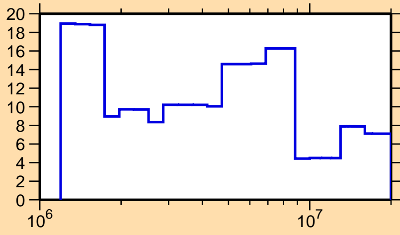
\Delta\sigma/\sigma vs. E for ^{208}\text{At}(n, \text{el.})
