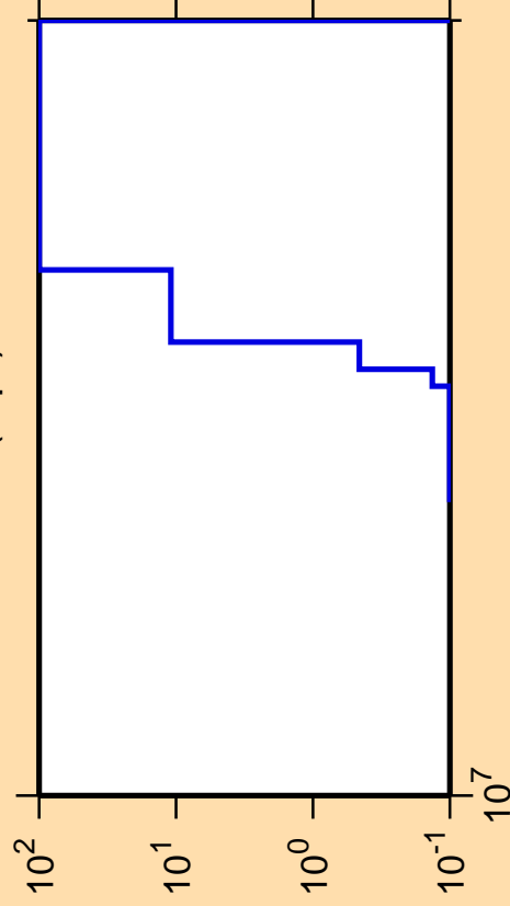
\Delta\sigma/\sigma vs. E for ^{208}\text{At}(n,pt)
