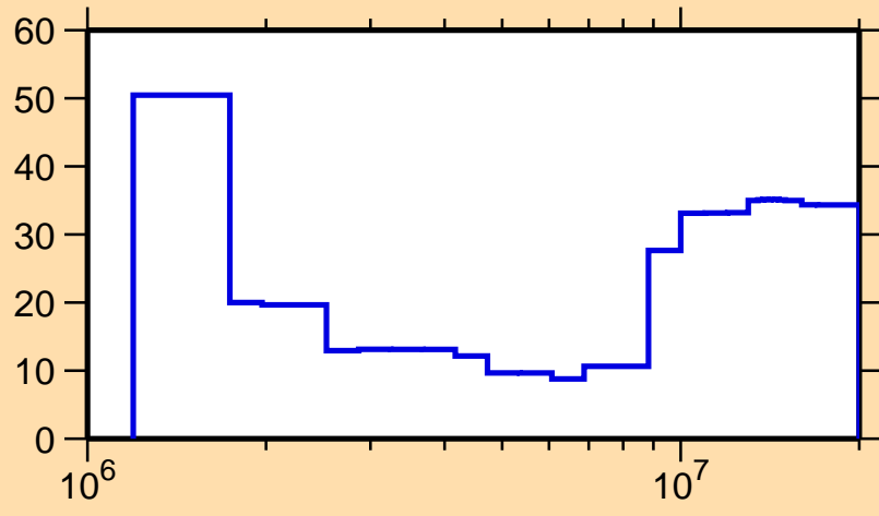
\Delta\sigma/\sigma vs. E for ^{208}\text{At}(n,n\text{cont.})
