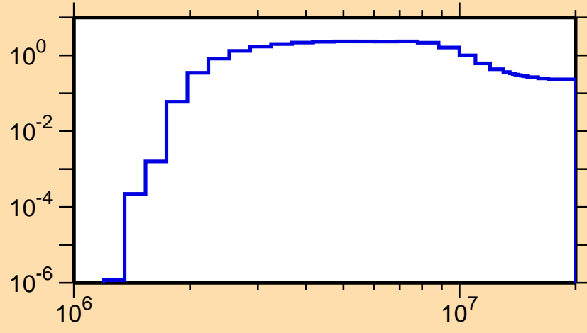
\sigma vs. E for ^{208}\text{At}(n,n\text{cont.})
