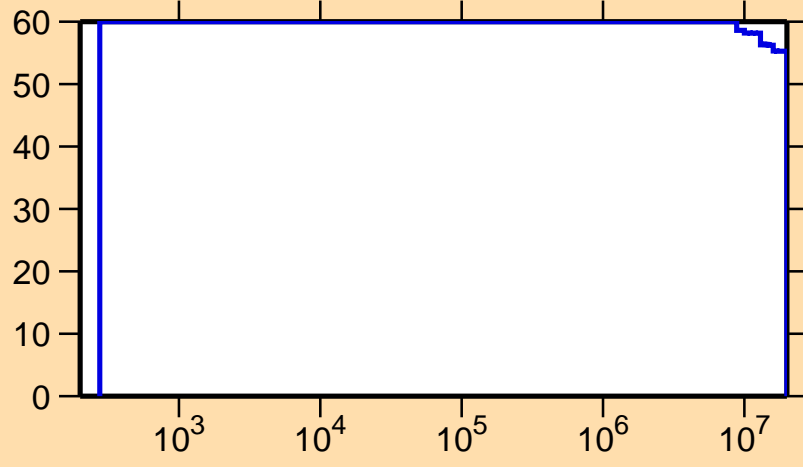
\Delta\sigma/\sigma vs. E for ^{208}\text{At}(n, p)
