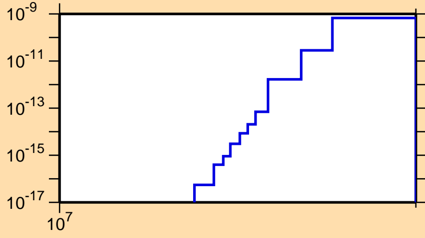
\sigma vs. E for ^{208}\text{At}(n,pt)
