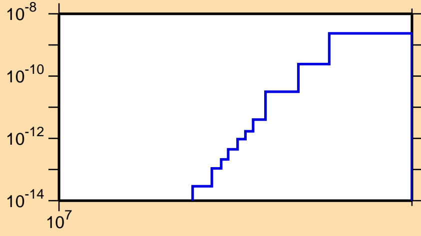
\sigma vs. E for ^{208}\text{At}(n,\text{pd})
