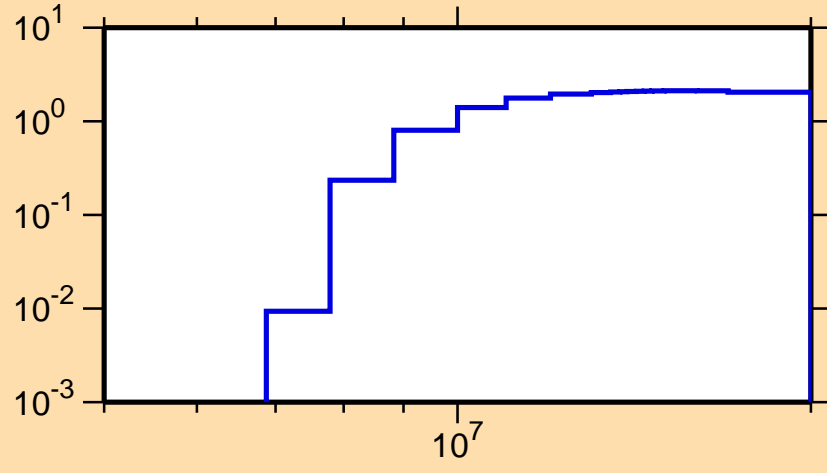
\sigma vs. E for ^{208}\text{At}(n,2n)
