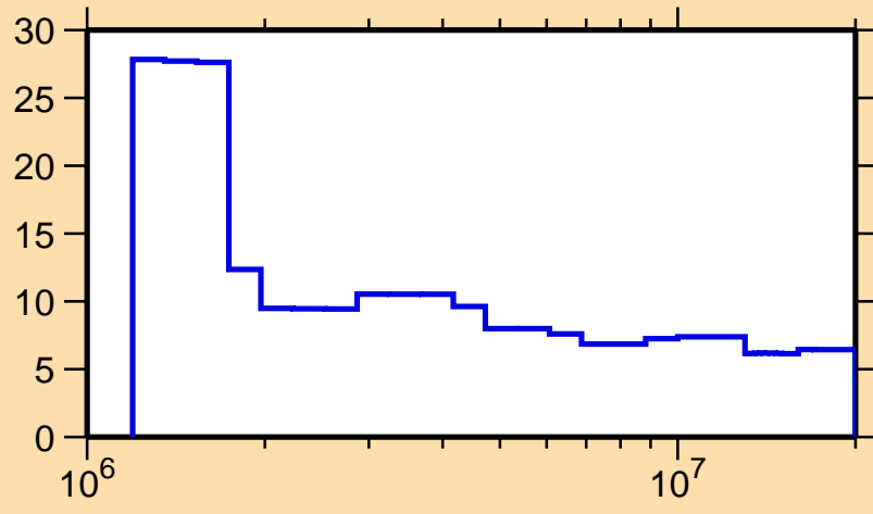
\Delta\sigma/\sigma vs. E for ^{208}\text{At}(n,\text{nonel.})
