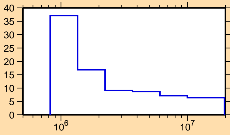
\Delta\sigma/\sigma vs. E for ^{208}\text{At}(n,n\text{nonel.})
