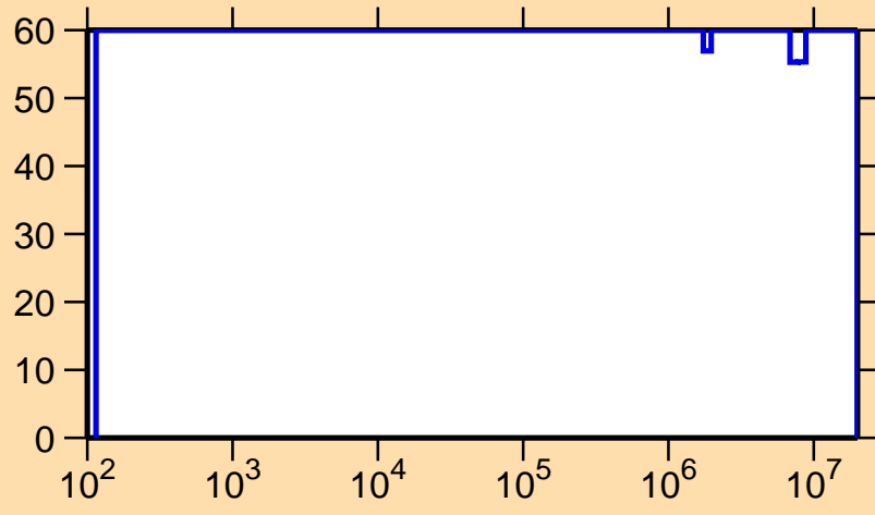
\Delta\sigma/\sigma vs. E for ^{209}\text{At}(n,\gamma)
