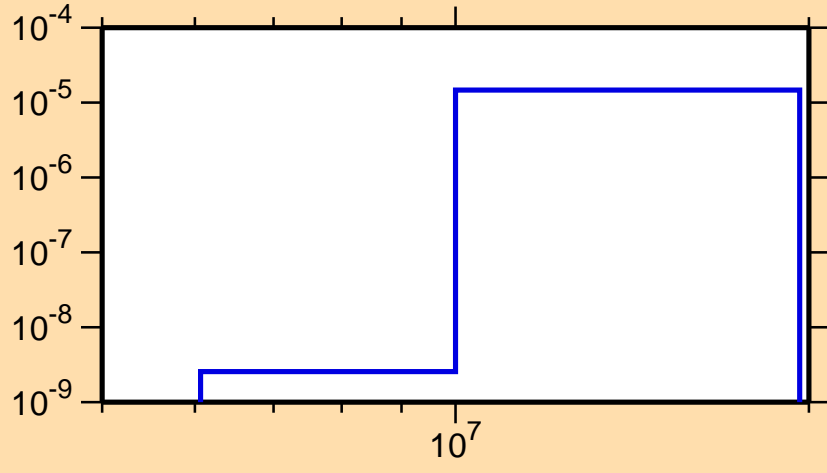
\sigma vs. E for ^{209}\text{At}(\text{mt117})
