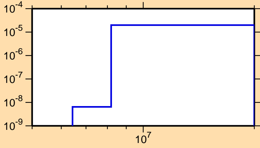
\sigma vs. E for ^{209}\text{At}(\text{mt } 45)
