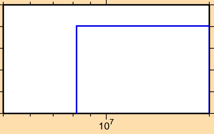
\sigma vs. E for ^{209}\text{At}(n,3n)
