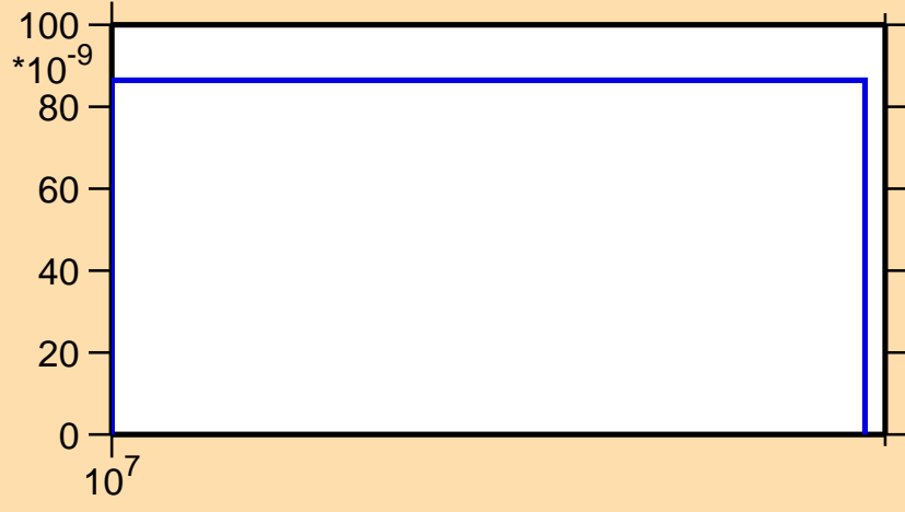
\sigma vs. E for ^{210}\text{At}(n,3n\alpha)
