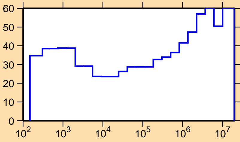
\Delta\sigma/\sigma vs. E for ^{210}\text{At}(n,\gamma)
