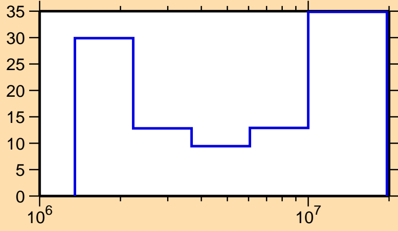
\Delta\sigma/\sigma vs. E for ^{210}\text{At}(n,n\text{cont.})
