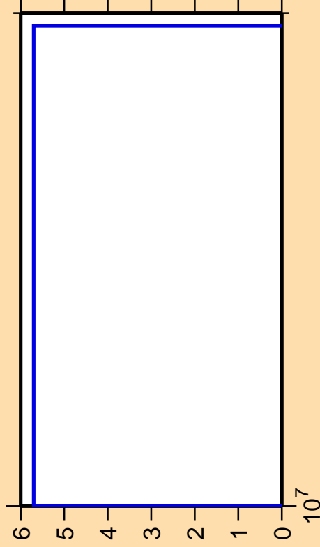
\Delta\sigma/\sigma vs. E for ^{210}\text{At}(n,\text{pt})
