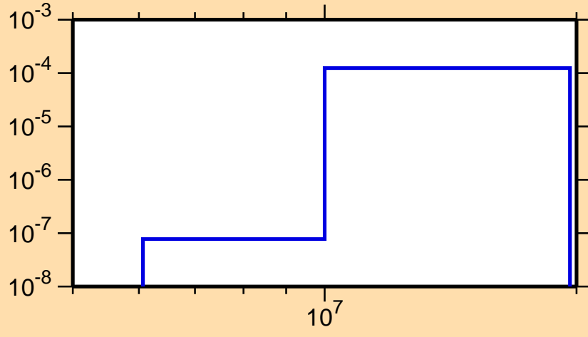
\sigma vs. E for ^{210}\text{At}(\text{mt } 45)
