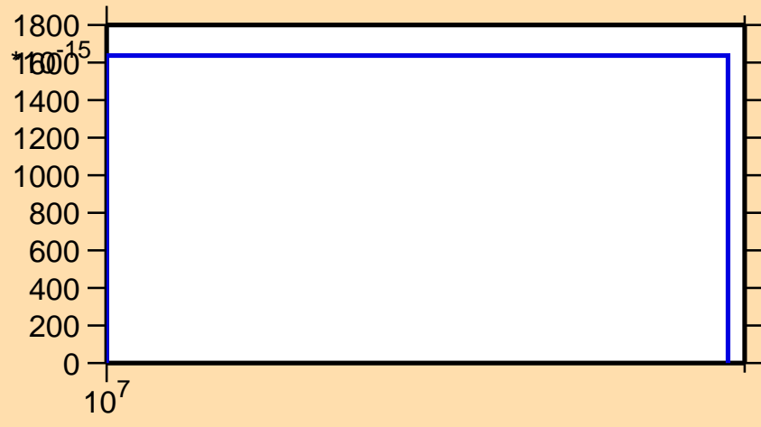
\sigma vs. E for ^{210}\text{At}(n,\text{pt})
