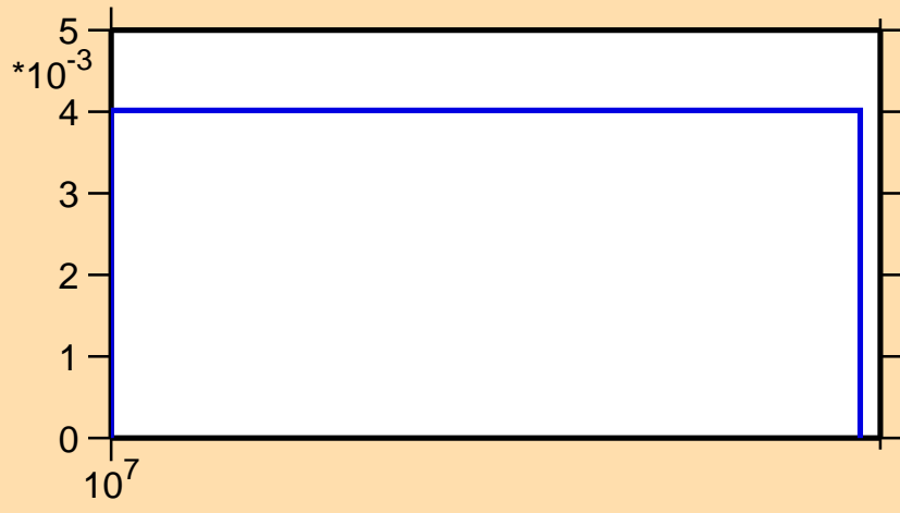
\sigma vs. E for ^{210}\text{At}(n,3n)
