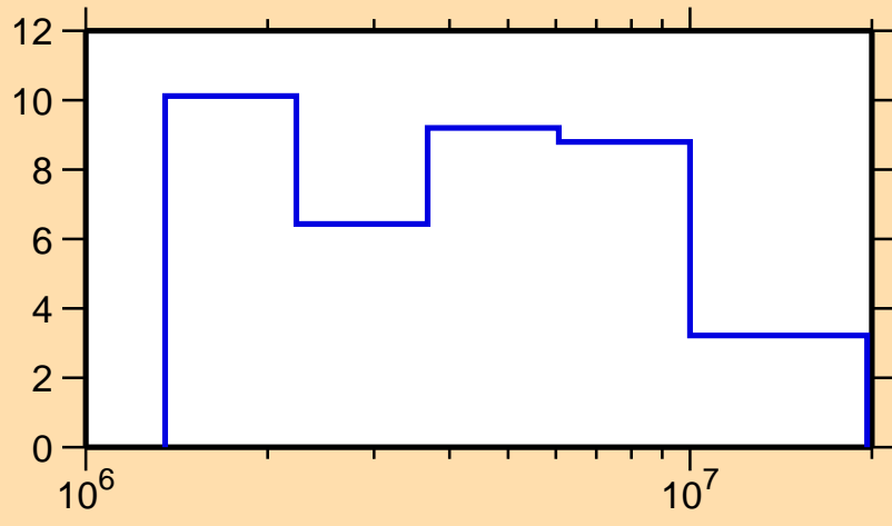
\Delta\sigma/\sigma vs. E for ^{210}\text{At}(n,\text{tot.})
