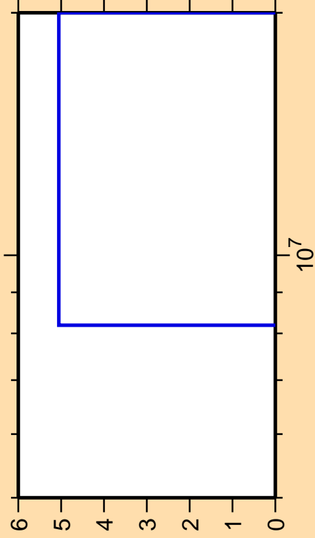
\Delta\sigma/\sigma vs. E for ^{210}\text{At}(n,pt)
