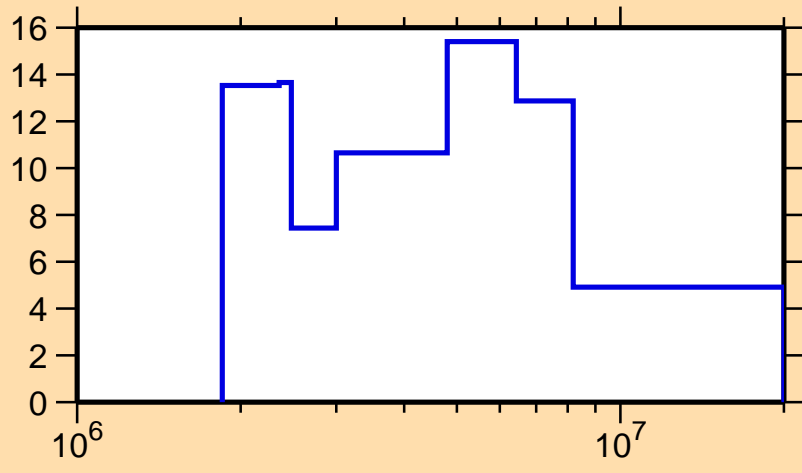
\Delta\sigma/\sigma vs. E for ^{210}\text{At}(n, el.)
