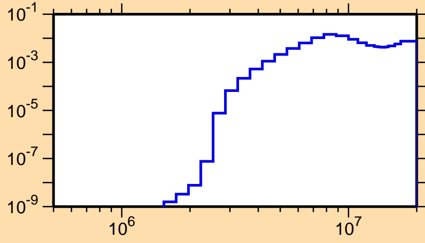
\sigma vs. E for ^{211}\text{At}(n,n\alpha)
