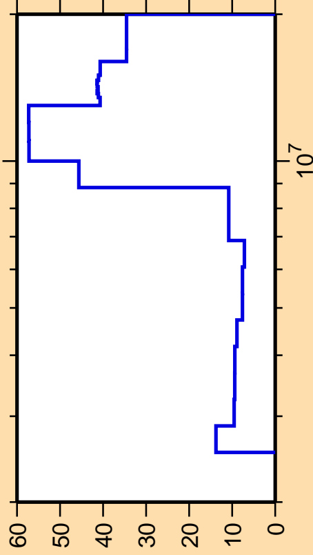
\Delta\sigma/\sigma vs. E for ^{211}\text{At}(n,\text{ncont.})
