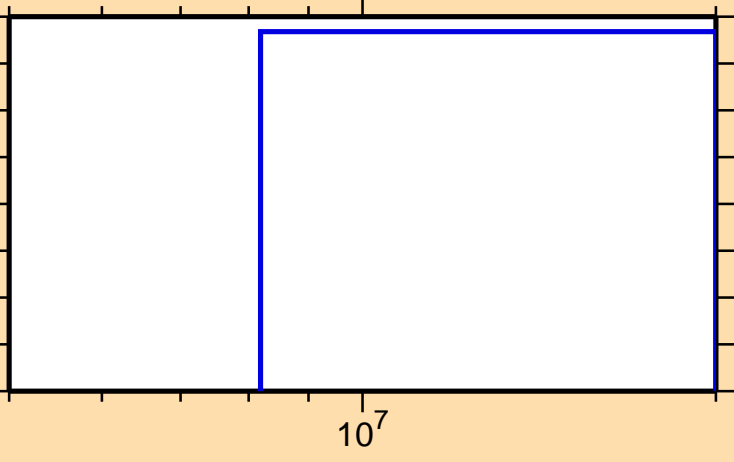
\sigma vs. E for ^{211}\text{At}(n,3n)
