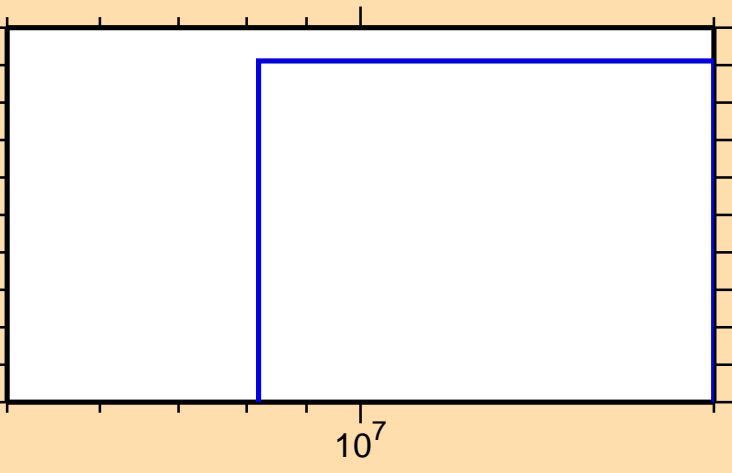
\sigma vs. E for ^{211}\text{At}(n,nt)
