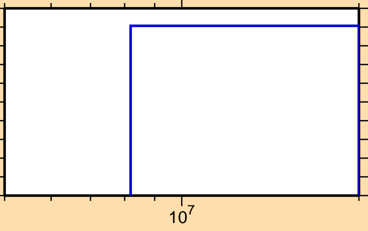
\sigma vs. E for ^{211}\text{At}(n,3n\alpha)
