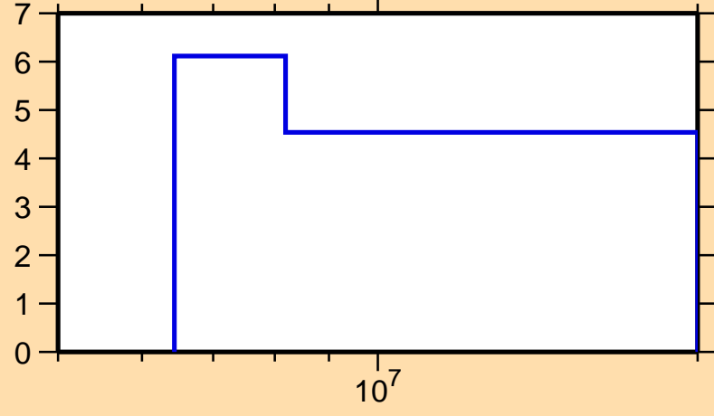
\Delta\sigma/\sigma vs. E for ^{211}\text{At}(n,\text{nonel.})
