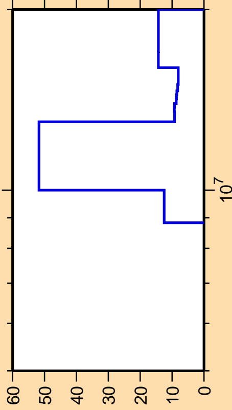
\Delta\sigma/\sigma vs. E for ^{219}\text{At}(n,3n\alpha)
