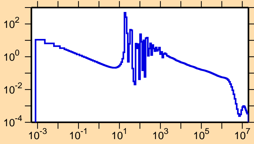
\sigma vs. E for ^{219}\text{At}(n,\gamma)
