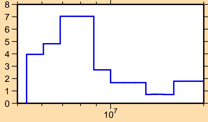
\Delta\sigma/\sigma vs. E for ^{219}\text{At}(n,\text{nonel.})
