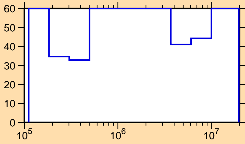
\Delta\sigma/\sigma vs. E for ^{219}\text{At}(n,n_1)
