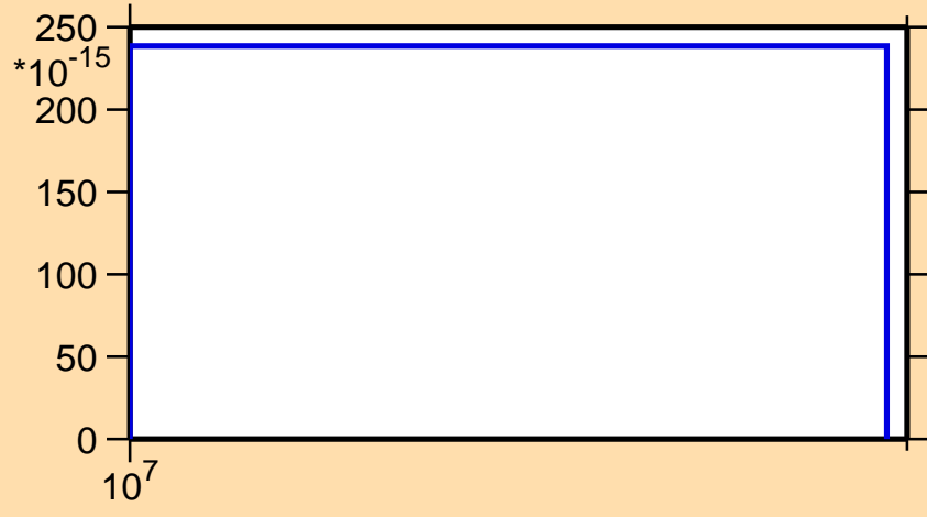
\sigma vs. E for ^{219}\text{At}(n,\text{He3})
