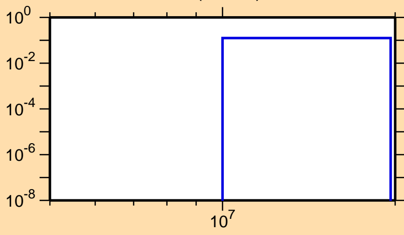
\sigma vs. E for ^{219}\text{At}(n,3n\alpha)
