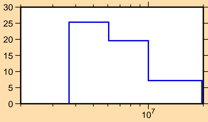
\Delta\sigma/\sigma vs. E for ^{219}\text{At}(n,el.)
