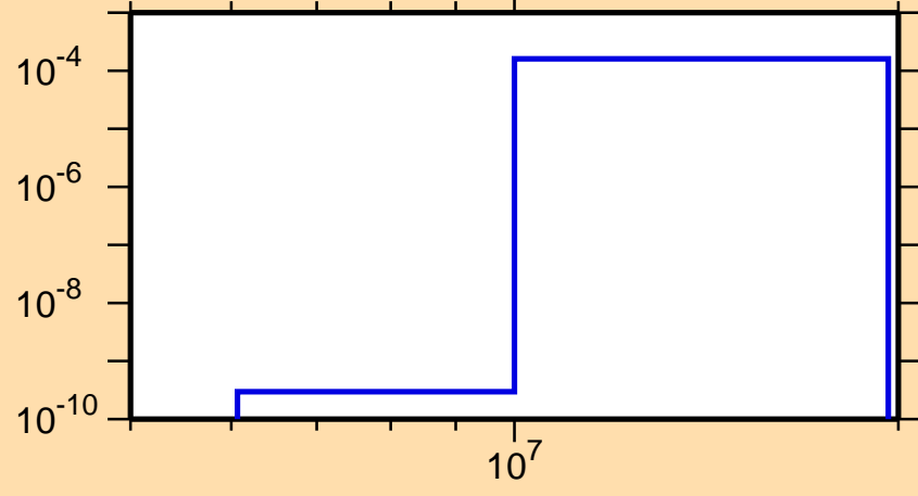
\sigma vs. E for ^{219}\text{At}(n,t)
