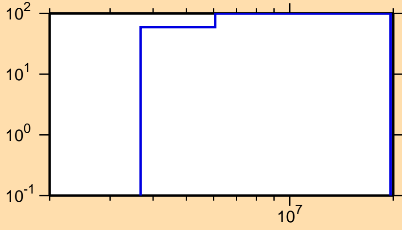
\Delta\sigma/\sigma vs. E for ^{219}\text{At}(n,ncont.)
