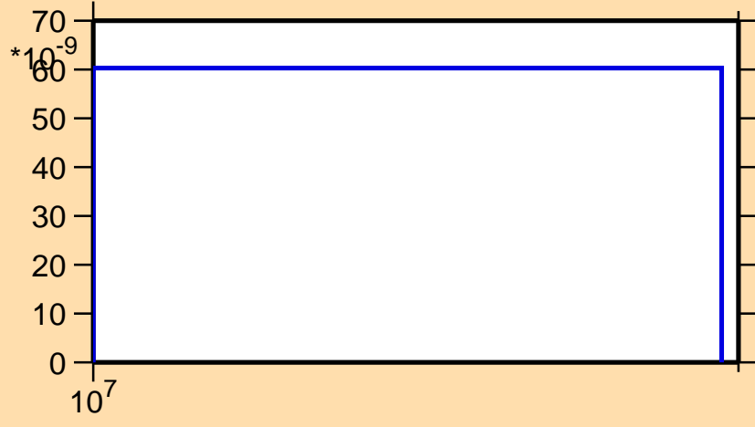
\sigma vs. E for ^{219}\text{At}(n,2np)
