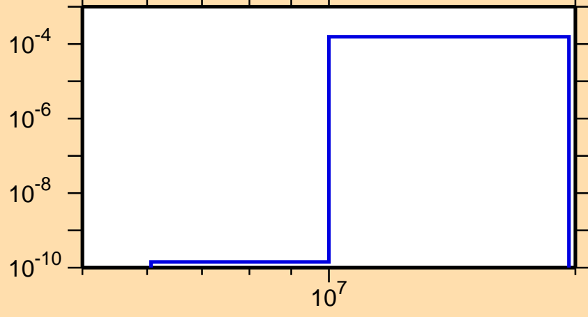
\sigma vs. E for ^{219}\text{At}(n,np)
