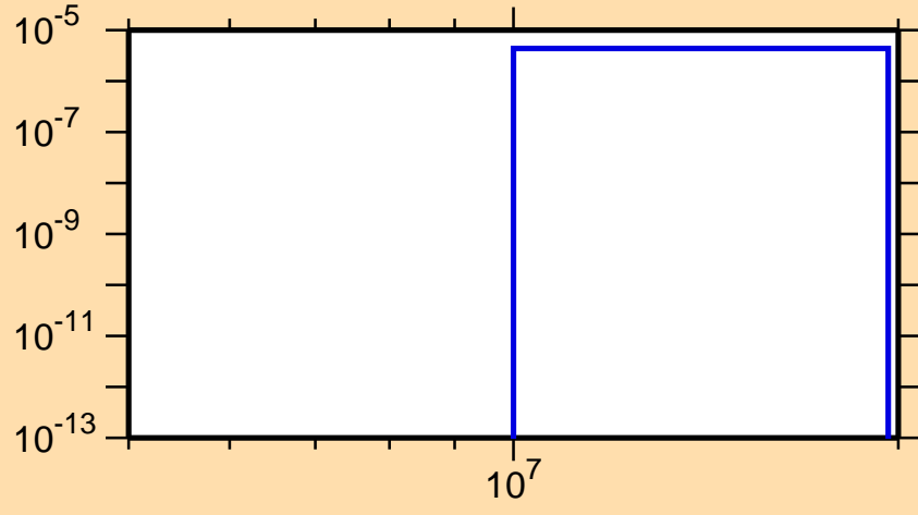
\sigma vs. E for ^{219}\text{At}(\text{mt } 45)
