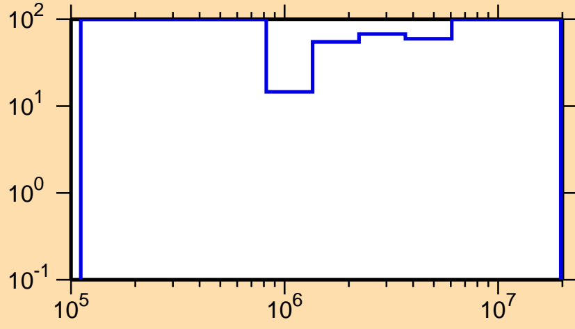
\Delta\sigma/\sigma vs. E for ^{219}\text{At}(n,n\text{cont.})
