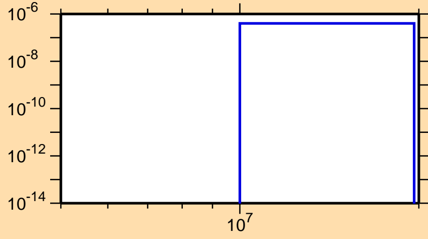
\sigma vs. E for ^{219}\text{At}(n,\text{nd})
