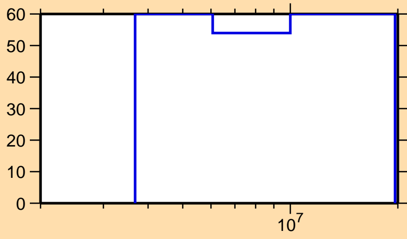
\Delta\sigma/\sigma vs. E for ^{219}\text{At}(n,\text{inel.})
