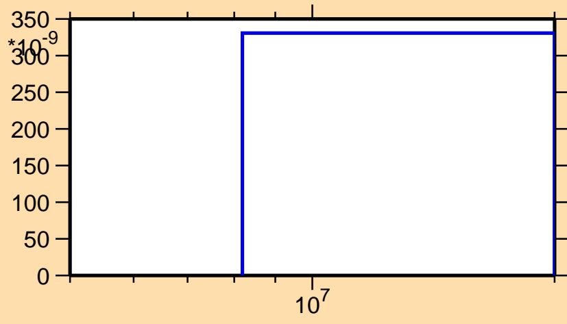
\sigma vs. E for ^{219}\text{At}(n,nd)
