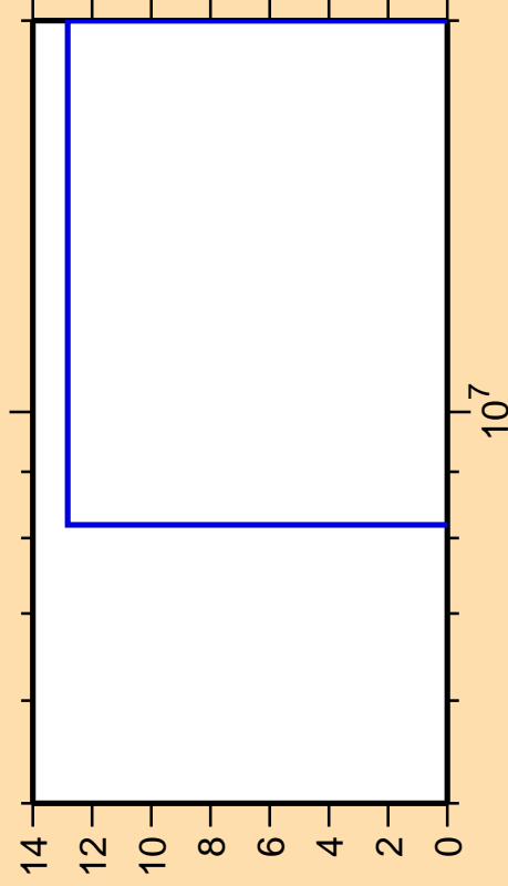
\Delta\sigma/\sigma vs. E for ^{219}\text{At}(n,nd)
