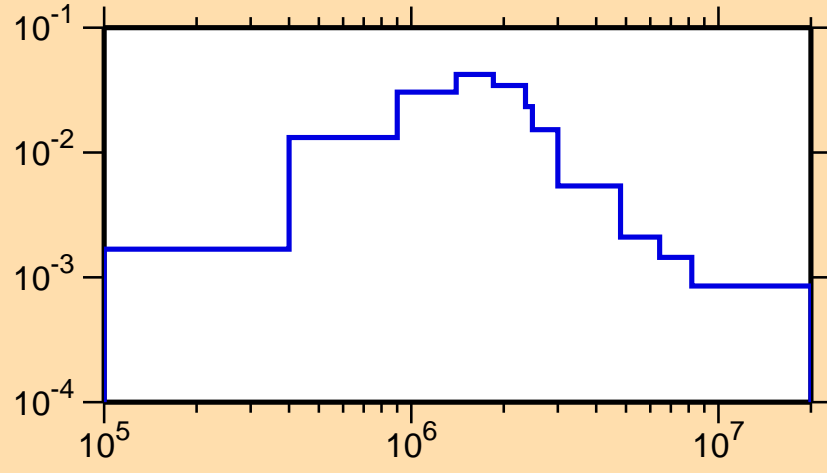
\sigma vs. E for ^{219}\text{At}(n,n_1)
