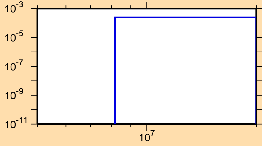
\sigma vs. E for ^{219}\text{At}(n,d)
