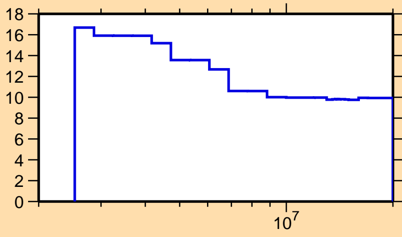
\Delta\sigma/\sigma vs. E for ^{220}\text{At}(n,\text{nonel.})
