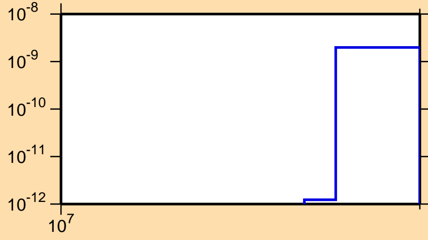
\sigma vs. E for ^{220}\text{At}(\text{mt } 11)
