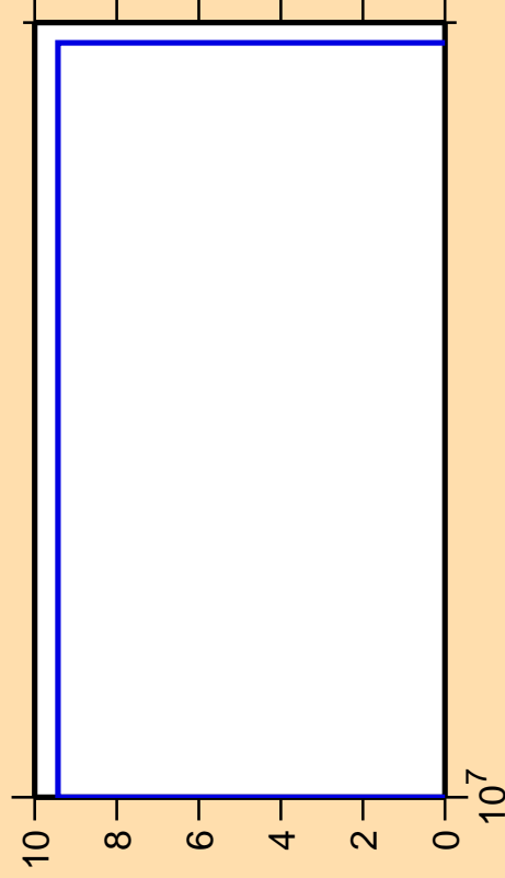
\Delta\sigma/\sigma vs. E for ^{220}\text{At} (mt 11)
