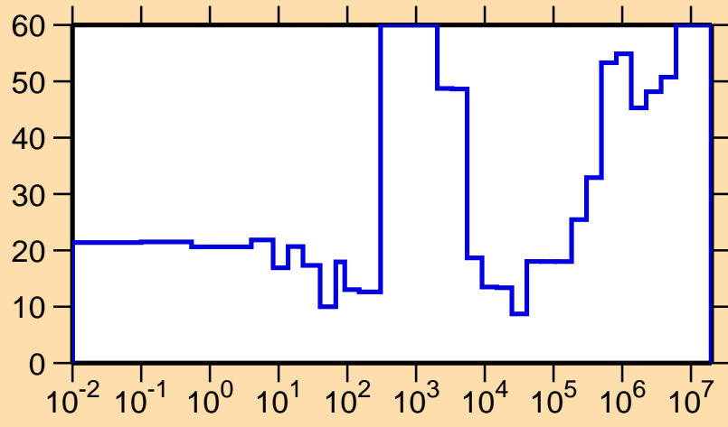
\Delta\sigma/\sigma vs. E for ^{220}\text{At}(n,el.)
