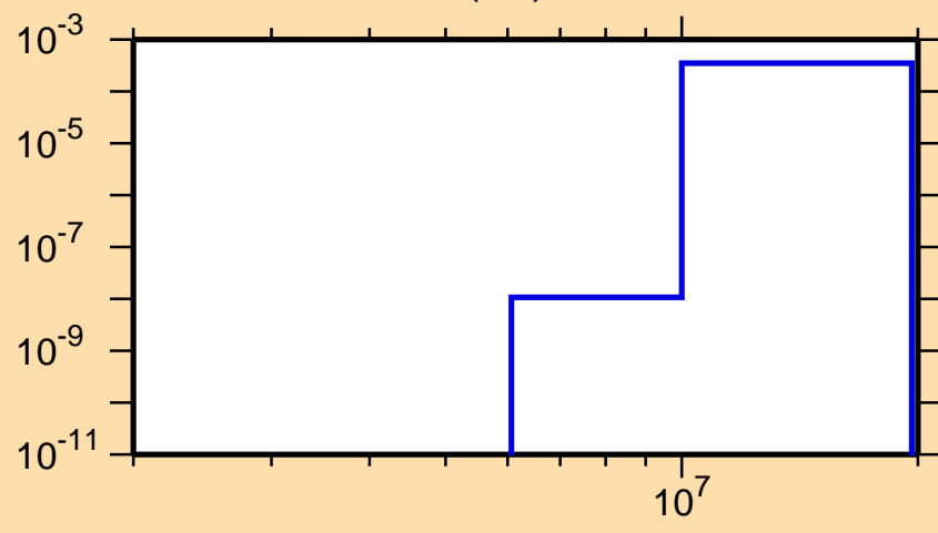
\sigma vs. E for ^{220}\text{At}(n,t)
