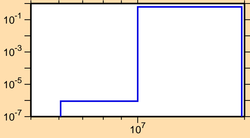
\sigma vs. E for ^{220}\text{At}(n,3n)
