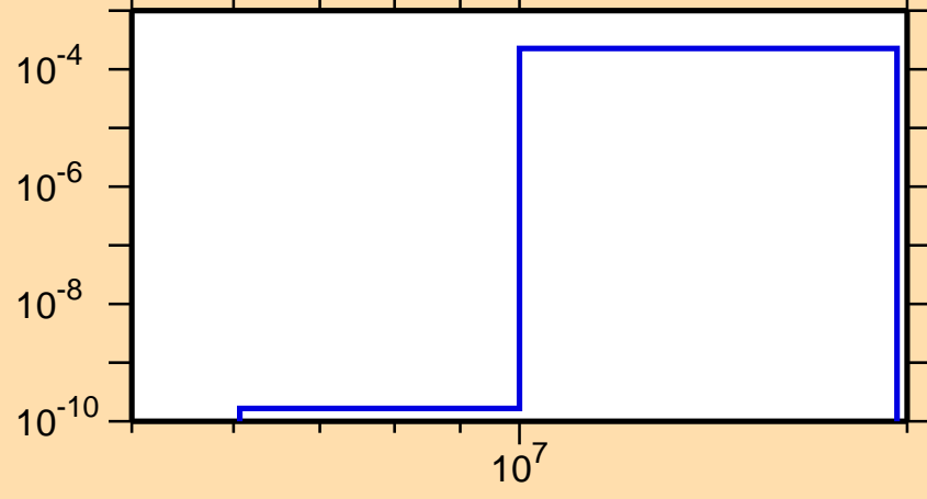
\sigma vs. E for ^{220}\text{At}(n,np)
