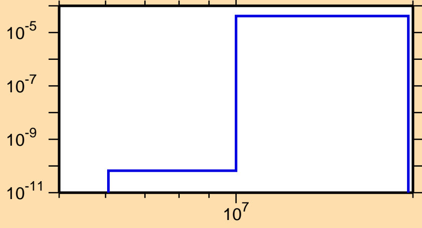
\sigma vs. E for ^{220}\text{At}(\text{mt117})
