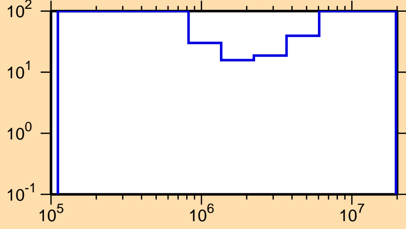
\Delta\sigma/\sigma vs. E for ^{220}\text{At}(n, ncont.)
