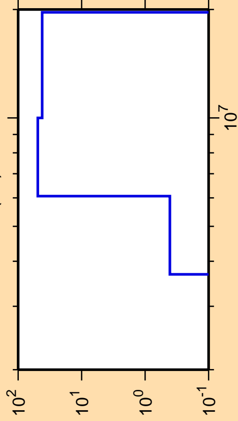
\Delta\sigma/\sigma vs. E for ^{220}\text{At}(n,t)
