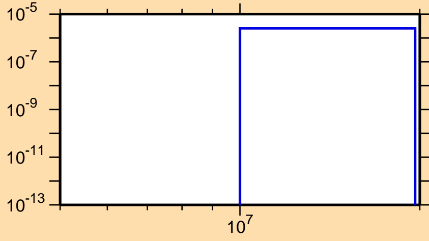
\sigma vs. E for ^{220}\text{At}(n,\text{nd})
