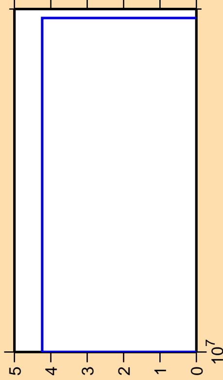
\Delta\sigma/\sigma vs. E for ^{220}\text{At} (mt 42)
