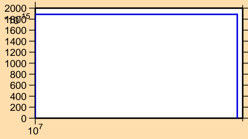
\sigma vs. E for ^{220}\text{At} (mt 42)
