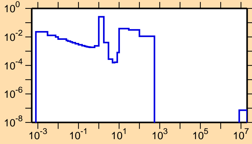
\sigma vs. E for ^{220}\text{At}(n,f)
