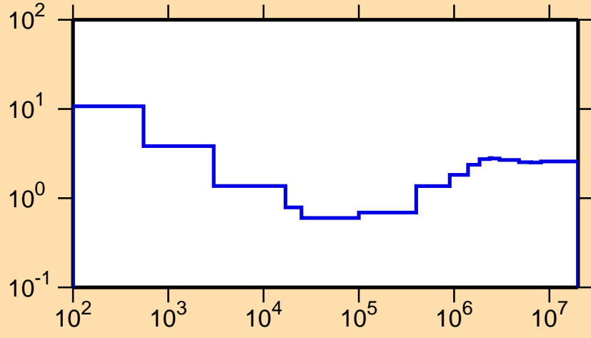
\sigma vs. E for ^{220}\text{At}(n,\text{nonel.})
