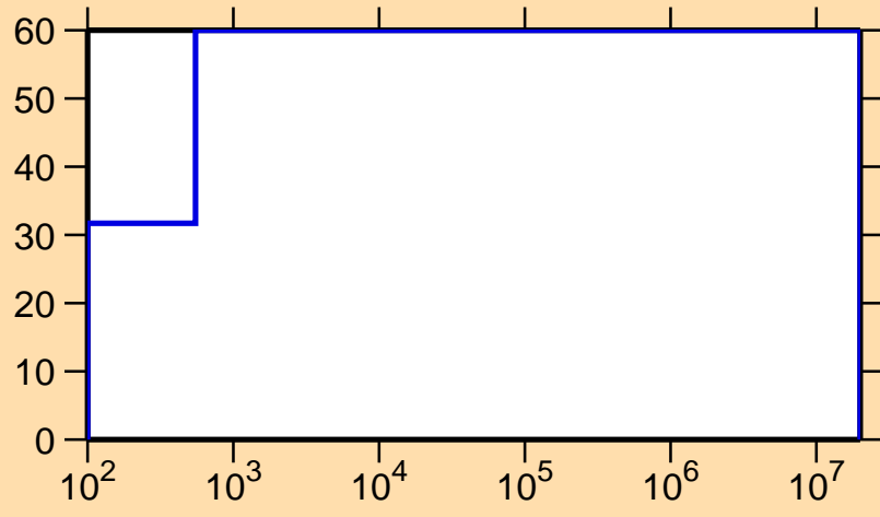
\Delta\sigma/\sigma vs. E for ^{220}\text{At}(n,\gamma)
