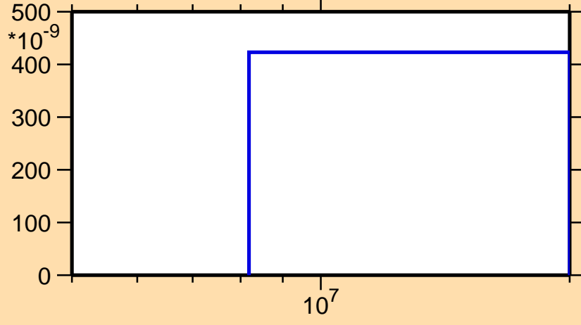
\sigma vs. E for ^{220}\text{At}(n,2np)
