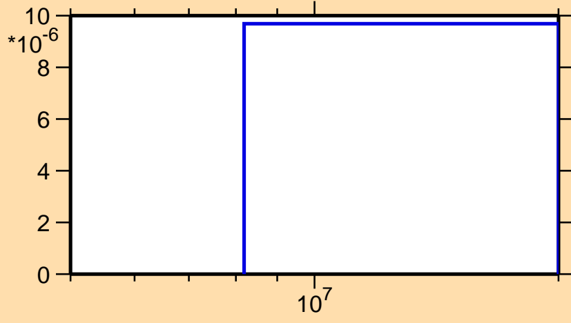
\sigma vs. E for ^{220}\text{At}(n,nt)
