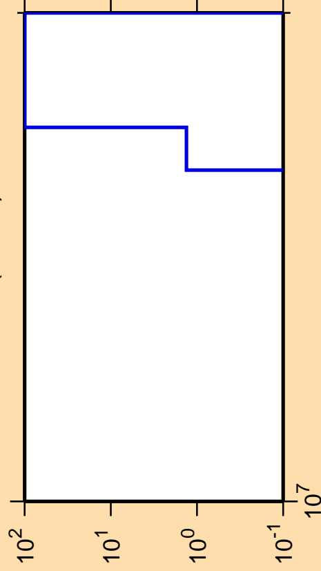
\Delta\sigma/\sigma vs. E for ^{221}\text{At} (mt 11)
