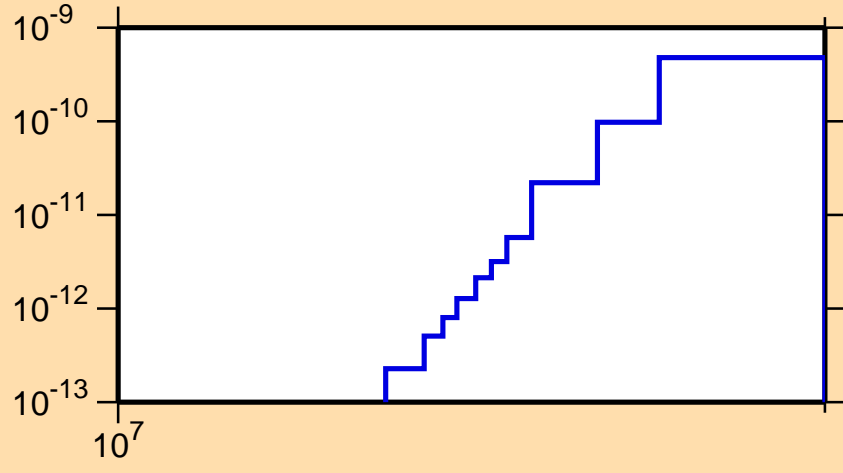
\sigma vs. E for ^{221}\text{At}(\text{mt } 45)
