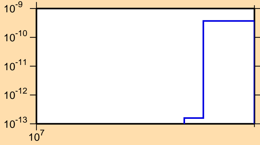
\sigma vs. E for ^{221}\text{At} (mt 11)
