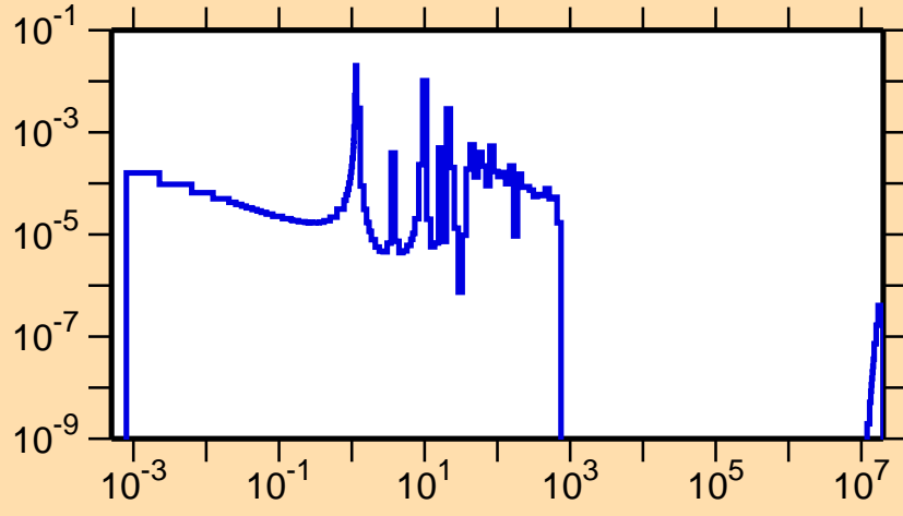
\sigma vs. E for ^{221}\text{At}(n,f)
