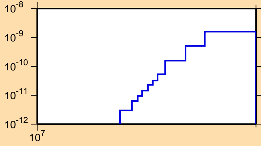
\sigma vs. E for ^{221}\text{At}(\text{mt117})
