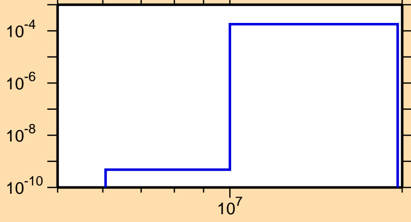
\sigma vs. E for ^{221}\text{At}(n,d)
